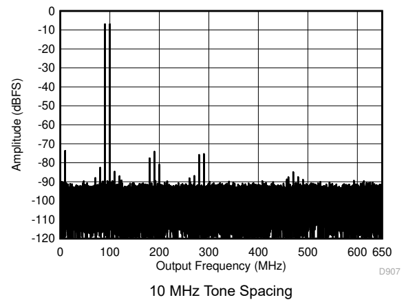
图 5-48. Two Tone FFT at 95.07 MHz Center
