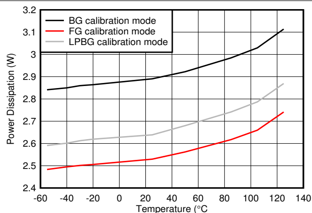
图 5-123. Quad Channel, Power Dissipation vs Temperature
