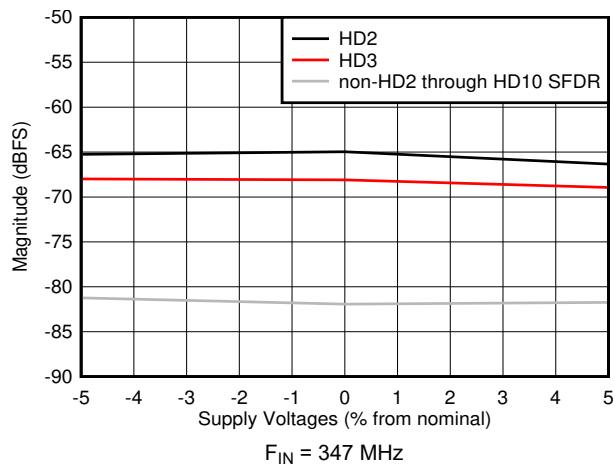
图 5-45. HD2, HD3 and Worst non-HD Spur vs Supply Voltage
