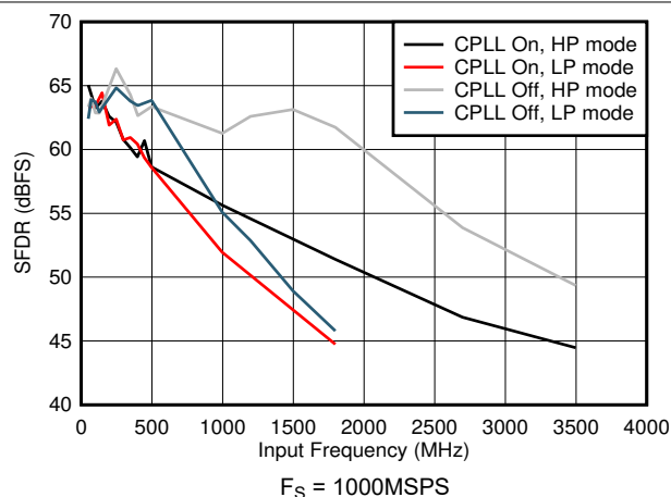
图 5-65. SFDR vs Input Frequency and CPLL
