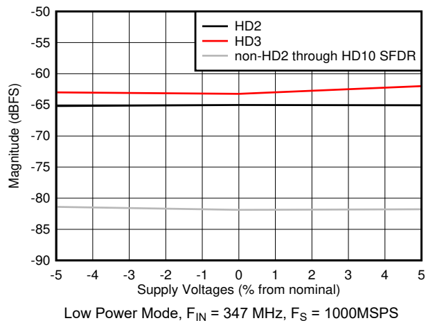
图 5-47. HD2, HD3 and Worst non-HD Spur vs Supply Voltage
