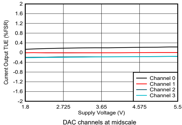
图 6-39. Current Output TUE vs Supply Voltage
