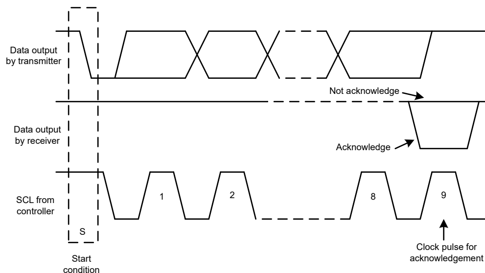
图 7-20. Acknowledge and Not Acknowledge on the I 2 C Bus
