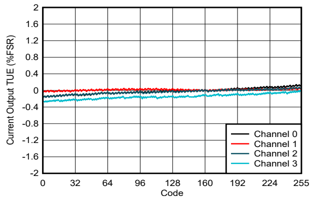
图 6-37. Current Output TUE vs Digital Input Code
