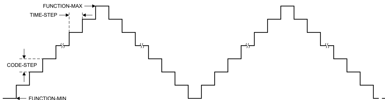
图 7-12. Triangle Waveform
