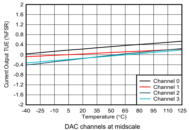
图 6-38. Current Output TUE vs Temperature
