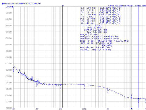
Figure 1. Closed-Loop Phase Noise of LVPECL Differential Output at 156.25 MHz
