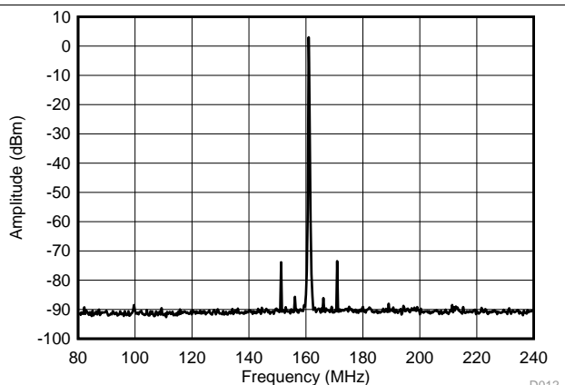
Figure 10. 161.1328125 ± 80.56640625-MHz LVPECL Differential Output Spectrum
