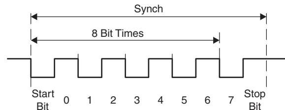
Figure 36-6. Auto Baud-Rate Detection – Synch Field
