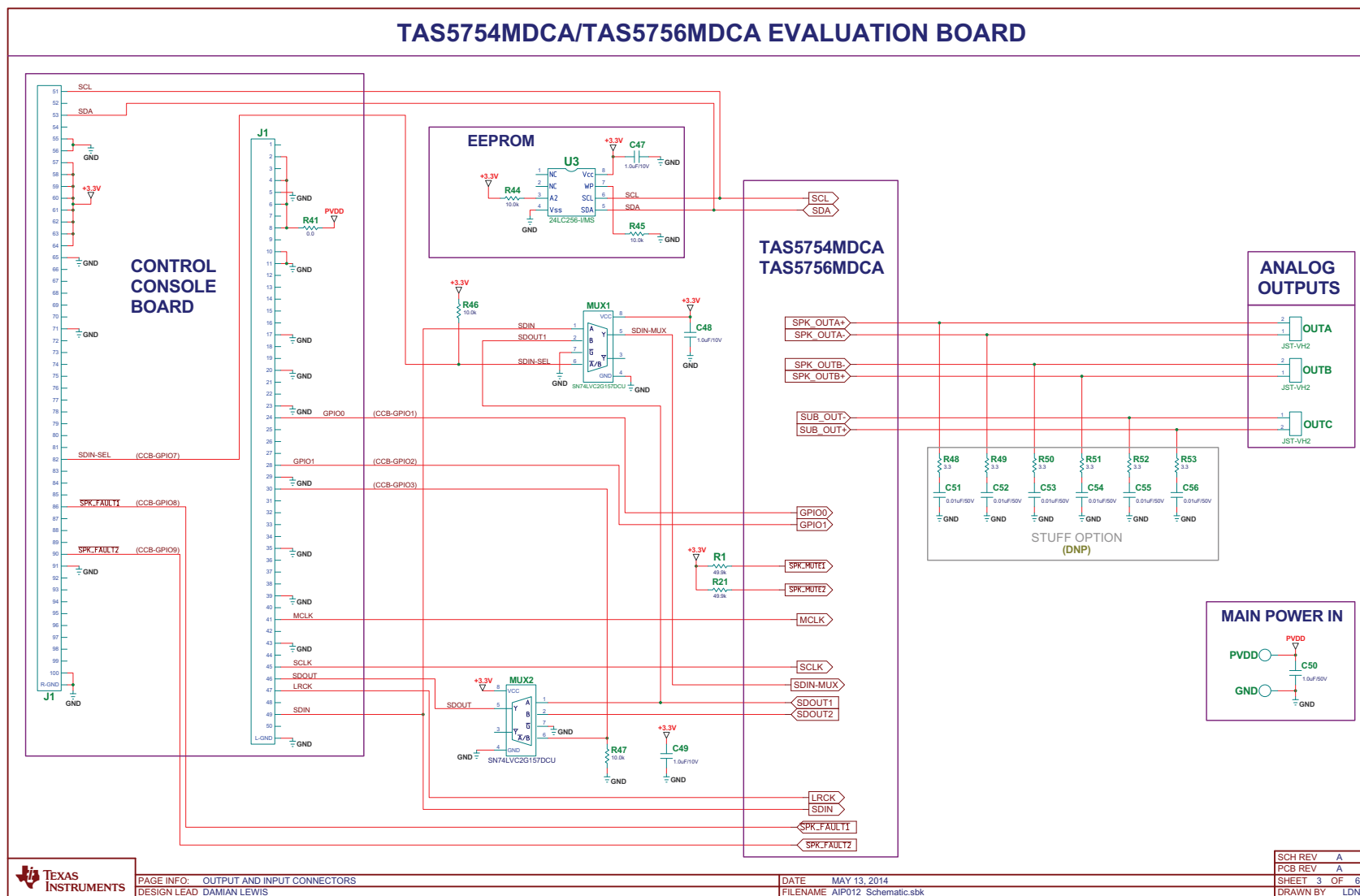
Figure 18. TAS5754/6MDCAEVM Schematic (Page 3 of 3)
