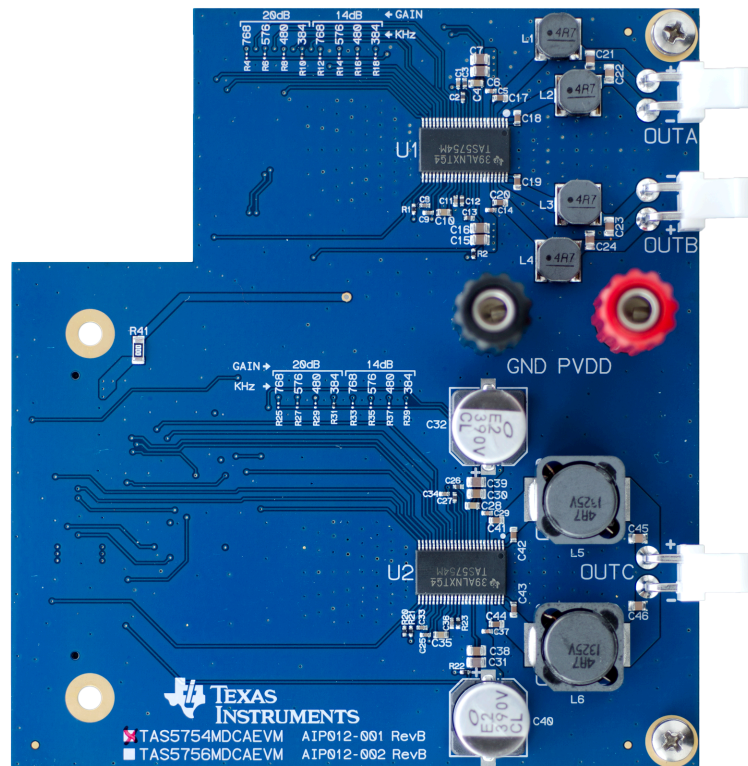
Figure 1. PPCMB and TAS5754/6MDCAEVM
