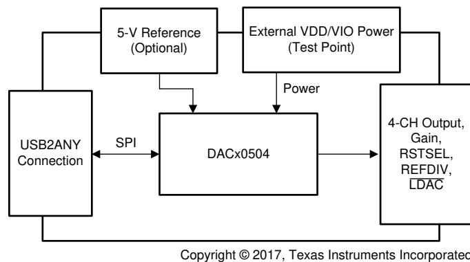
Figure 2. DACx0504EVM Block Diagram
