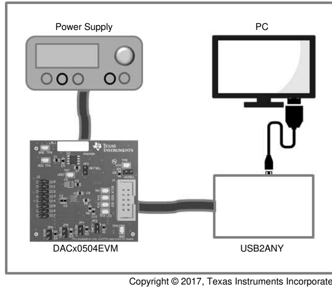
Figure 1. DACx0504EVM Hardware Setup
