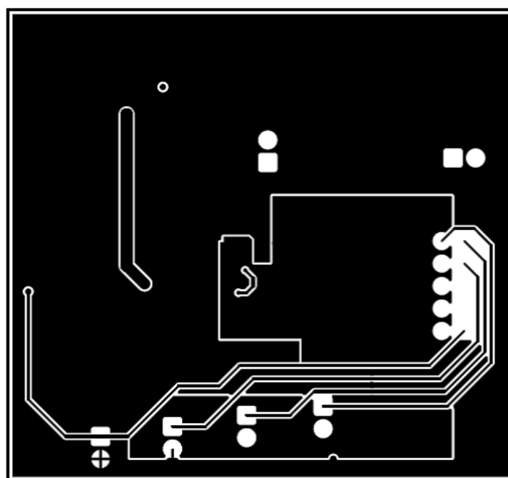
Figure 16. Bottom Layer
