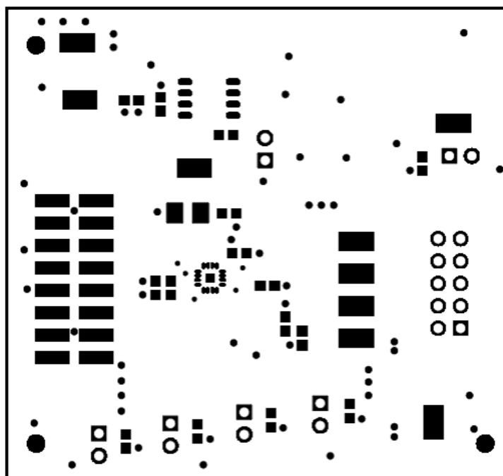
Figure 15. Top Solder
