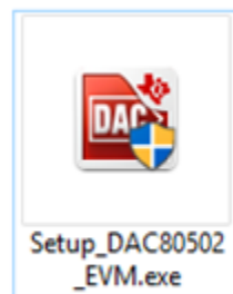
Figure 1. Software Setup
