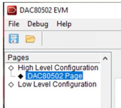
Figure 7. Page Selection
