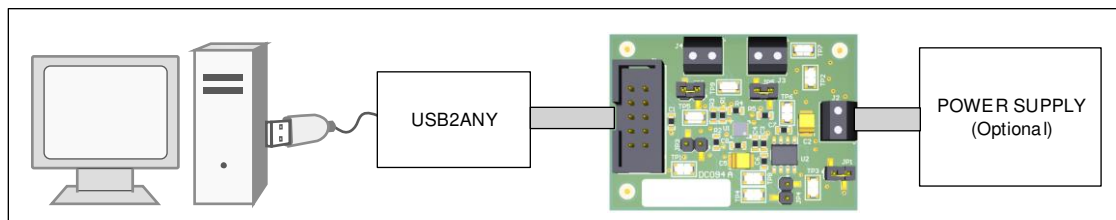
Figure 3. Hardware Setup
