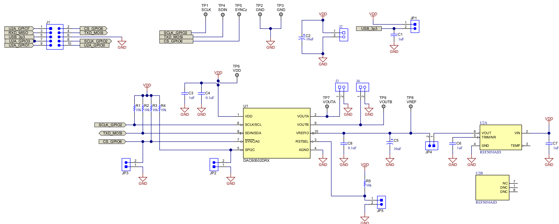
Figure 11. DAC80502EVM Schematic
