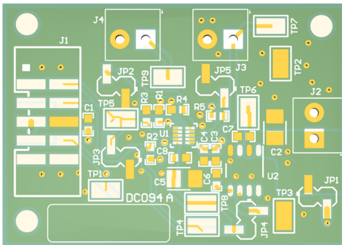
Figure 12. PCB Layout - Component Placement
