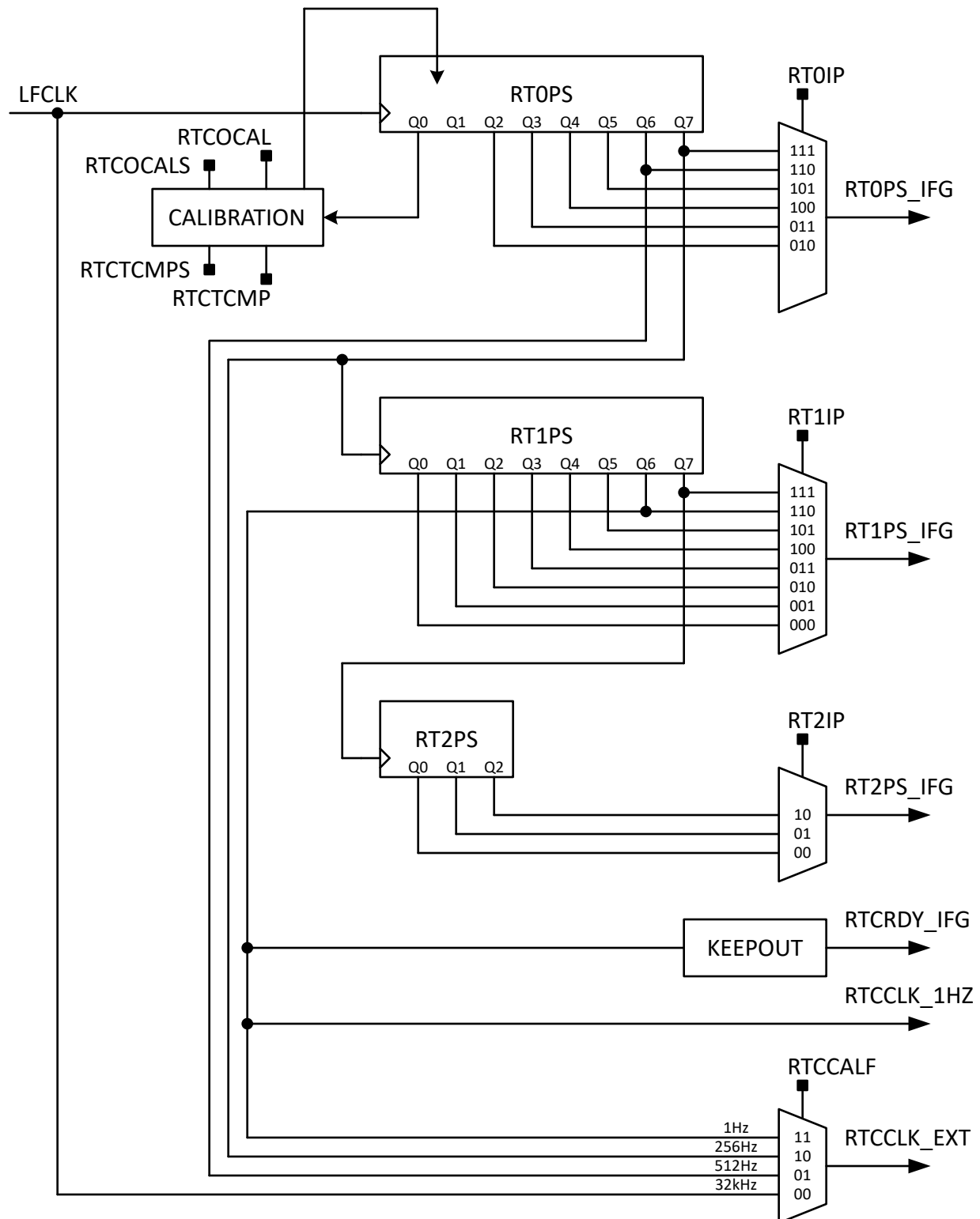
Figure 27-3. RTC Prescaler and Interval Timer Event
