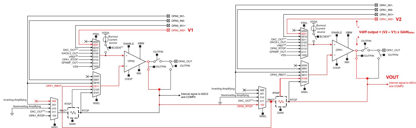
Figure 17-8. Two OPAs in Difference Amplifier Configuration
