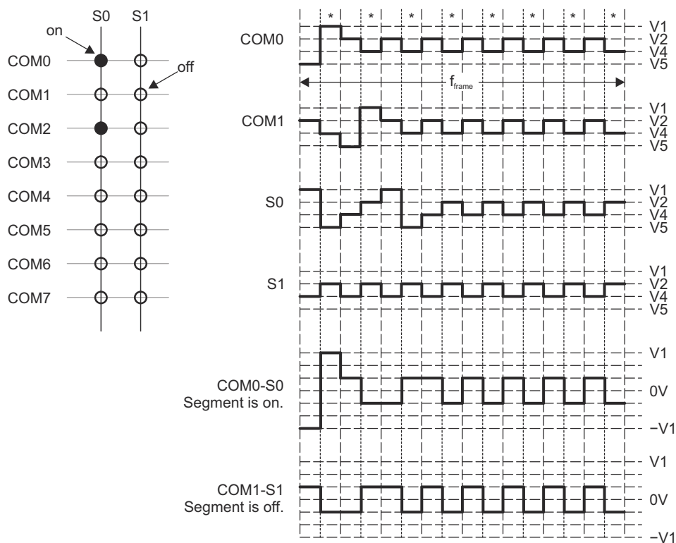
Figure 20-7. Example 8-Mux, 1/3 Bias Waveforms (LCDLP = 0)
