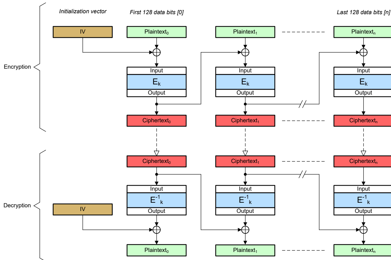
Figure 10-3. CBC Cipher
