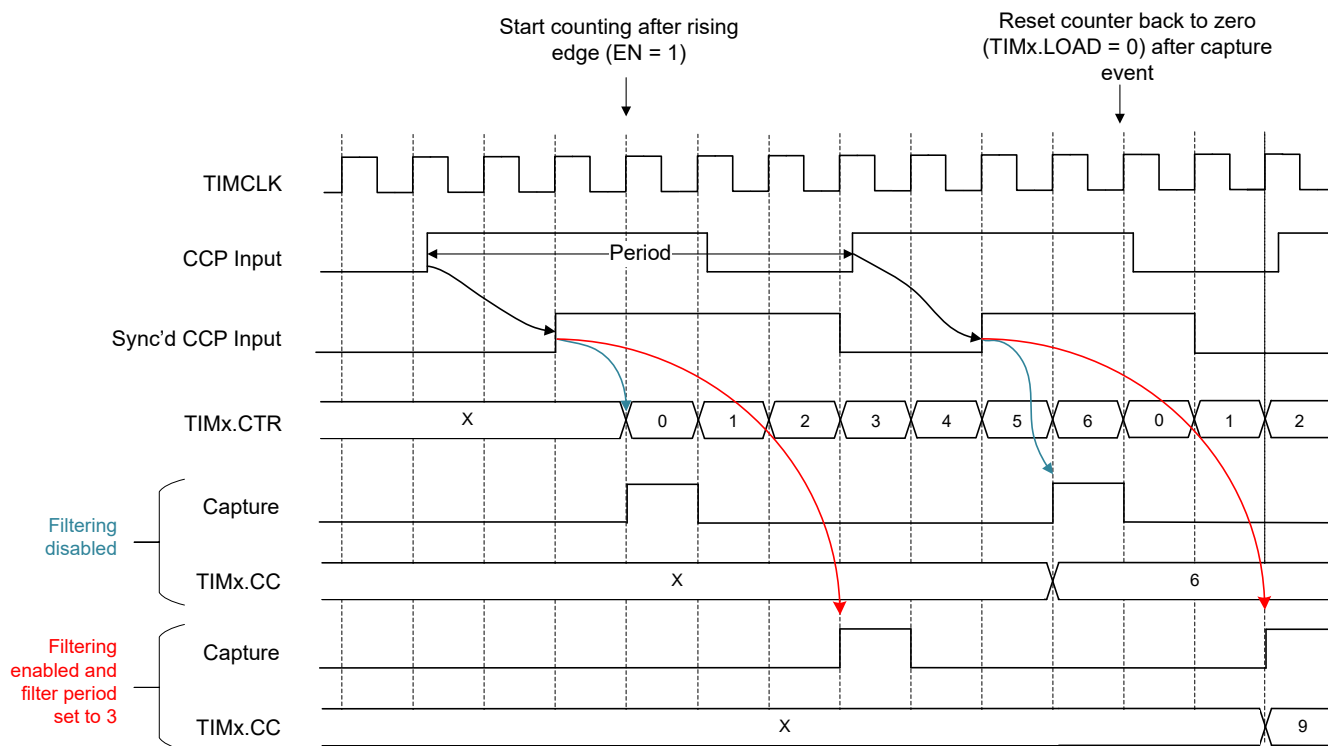
Figure 24-15. Period Capture Mode in Up-Counting Mode, CVAE = 2
