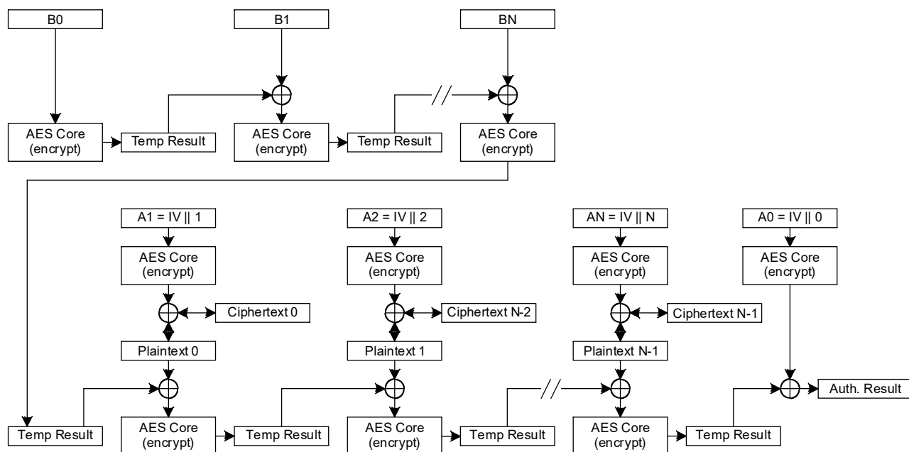
Figure 10-9. CCM Protocol Operation
