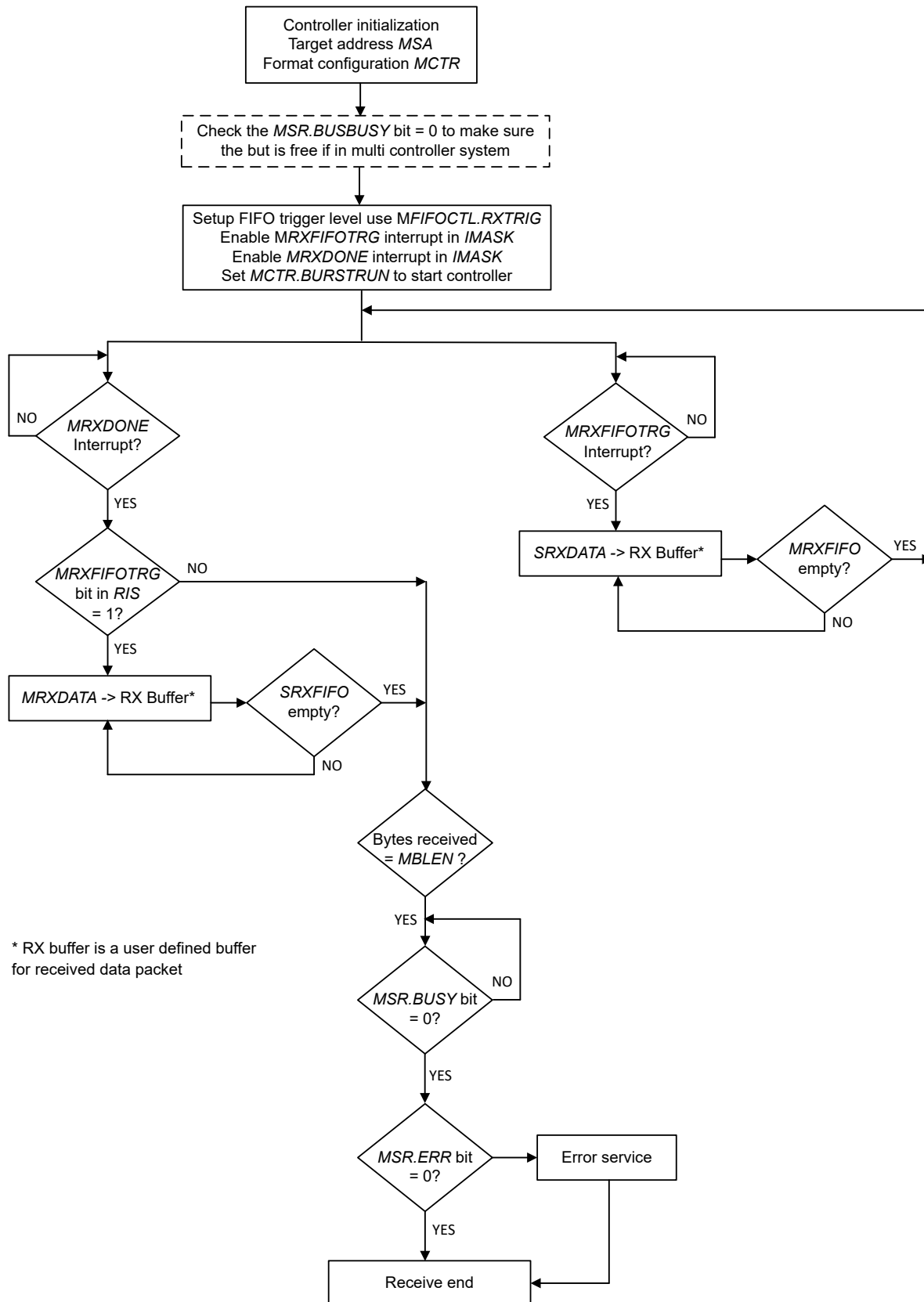
Figure 22-11. Controller Receiver Mode
