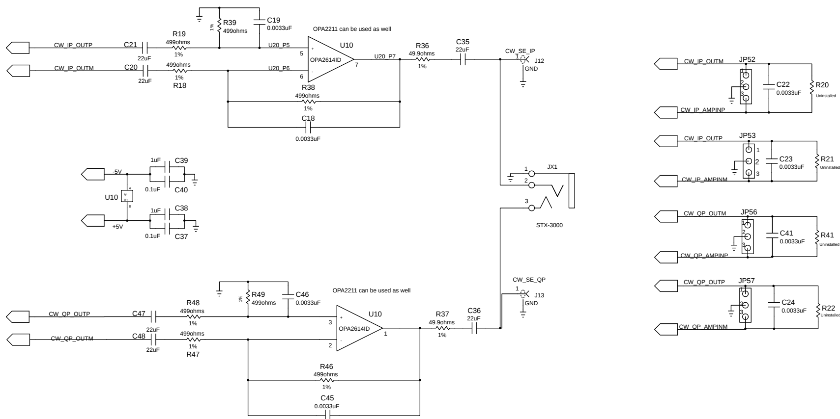
Figure 18. Schematic (Sheet 8 of 10)
