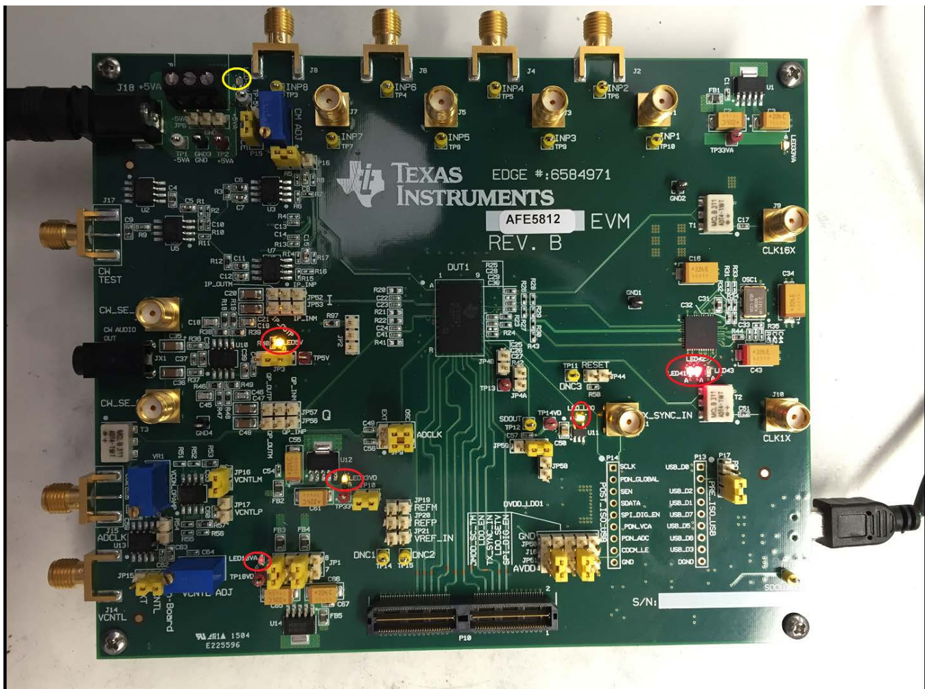
Figure 4. LED Placement
