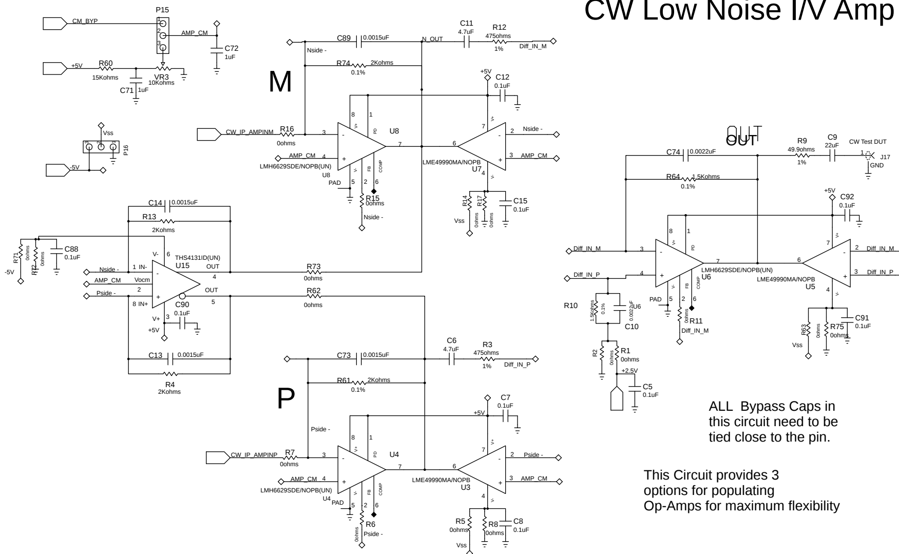
Figure 20. Schematic (Sheet 10 of 10)
