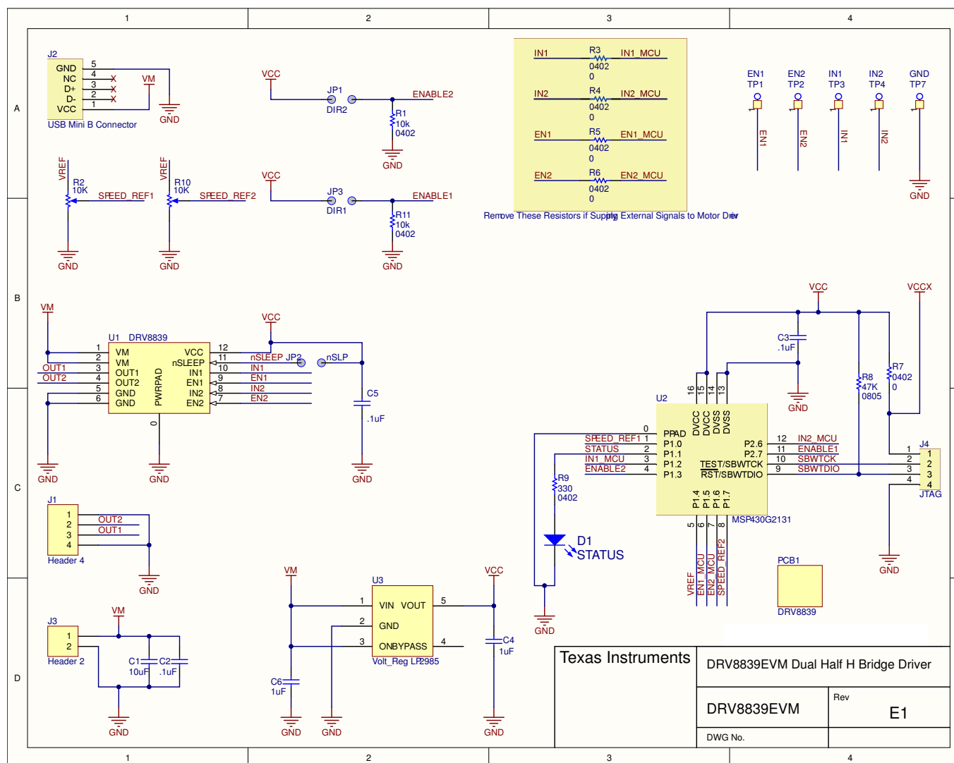
Figure 5. DRV8839EVM Schematic
