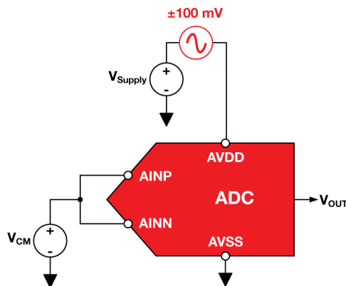
Figure 60. \text{PSRR}_{\text{AC}} measurement setup using a 100-mV P sine wave.
