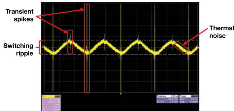
Figure 57. SMPS noise (transients, ripple and thermal noise).
