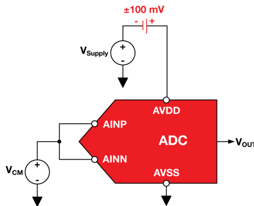
Figure 58. \text{PSRR}_{\text{DC}} measurement setup using \pm 100\text{-mV} offset on AVDD.
