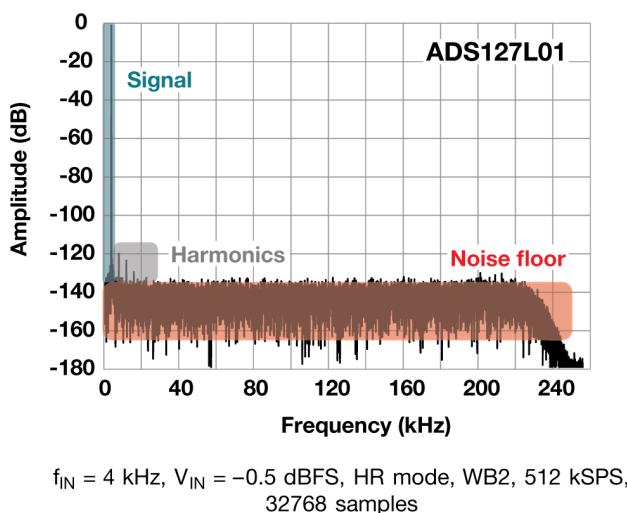
Figure 9. Example ADS127L01 FFT with a 4-kHz, -0.5-dBFS input signal.
