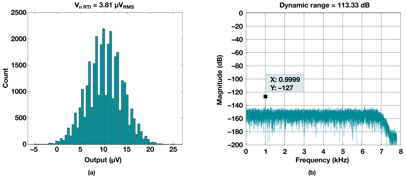
Figure 66. Noise histogram (a) and FFT (b) for clean supplies on LVDD and DVDD, ripple on AVDD.
