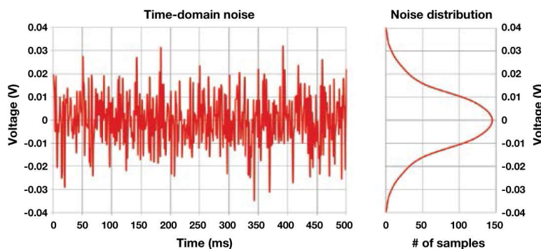
Figure 5. Thermal noise in the time domain with Gaussian distribution.
