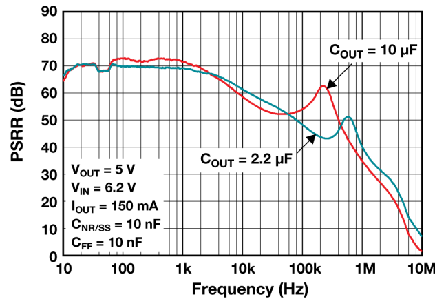
Figure 75. PSRR vs. frequency plot for the TPS7A49 LDO, C_{OUT} = 2.2 \mu F .
