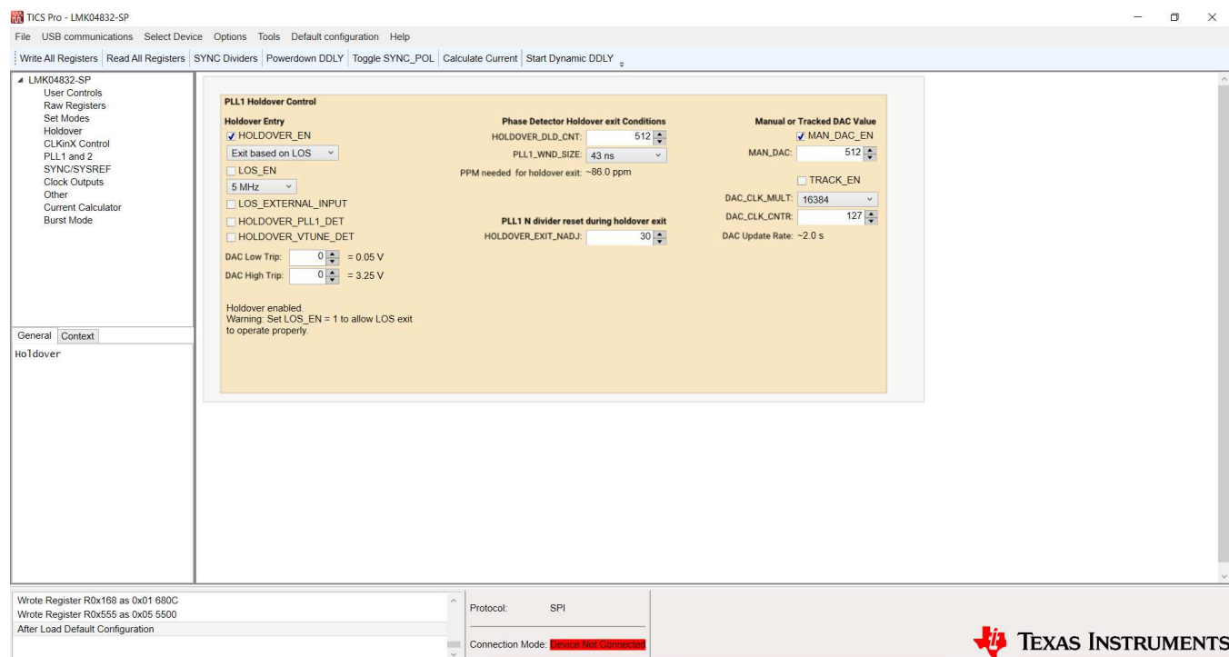
Figure 17. TICS Pro - Holdover Page
