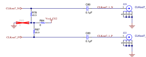
CLKout7
