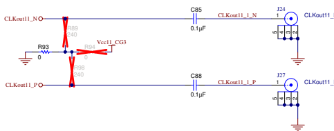
Figure 12. Schematic - Clock Outputs 2 of 2
