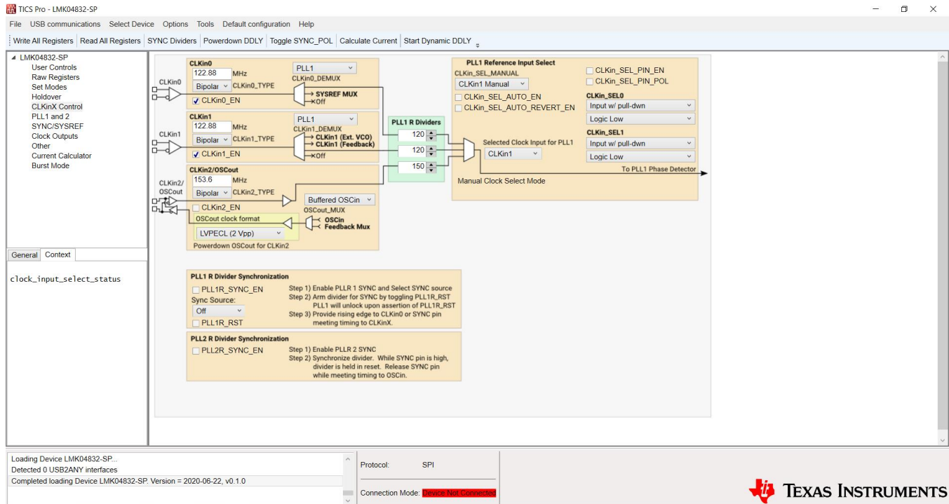
Figure 18. TICS Pro - CLKinX Control Page
