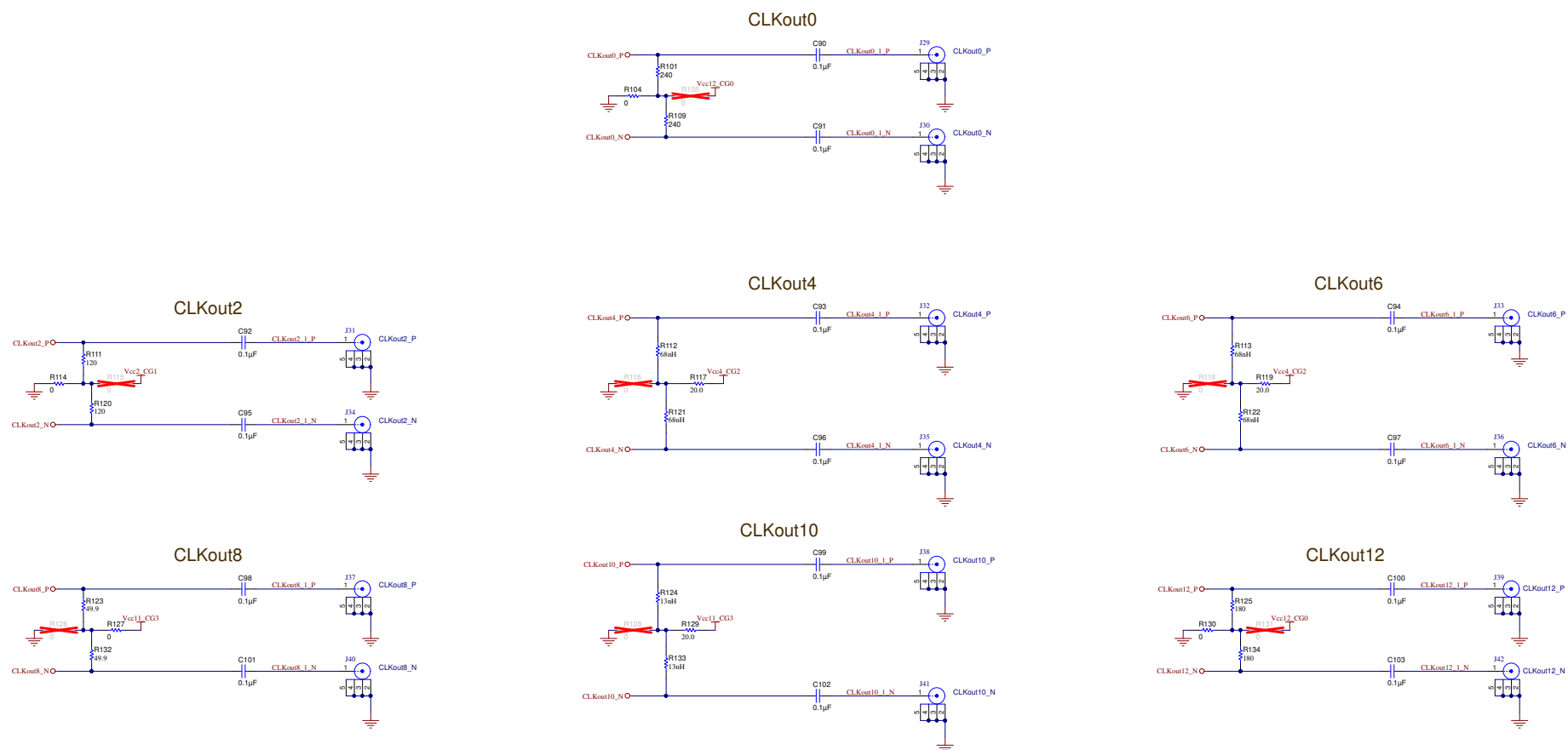
Figure 11. Schematic - Clock Outputs 1 of 2
