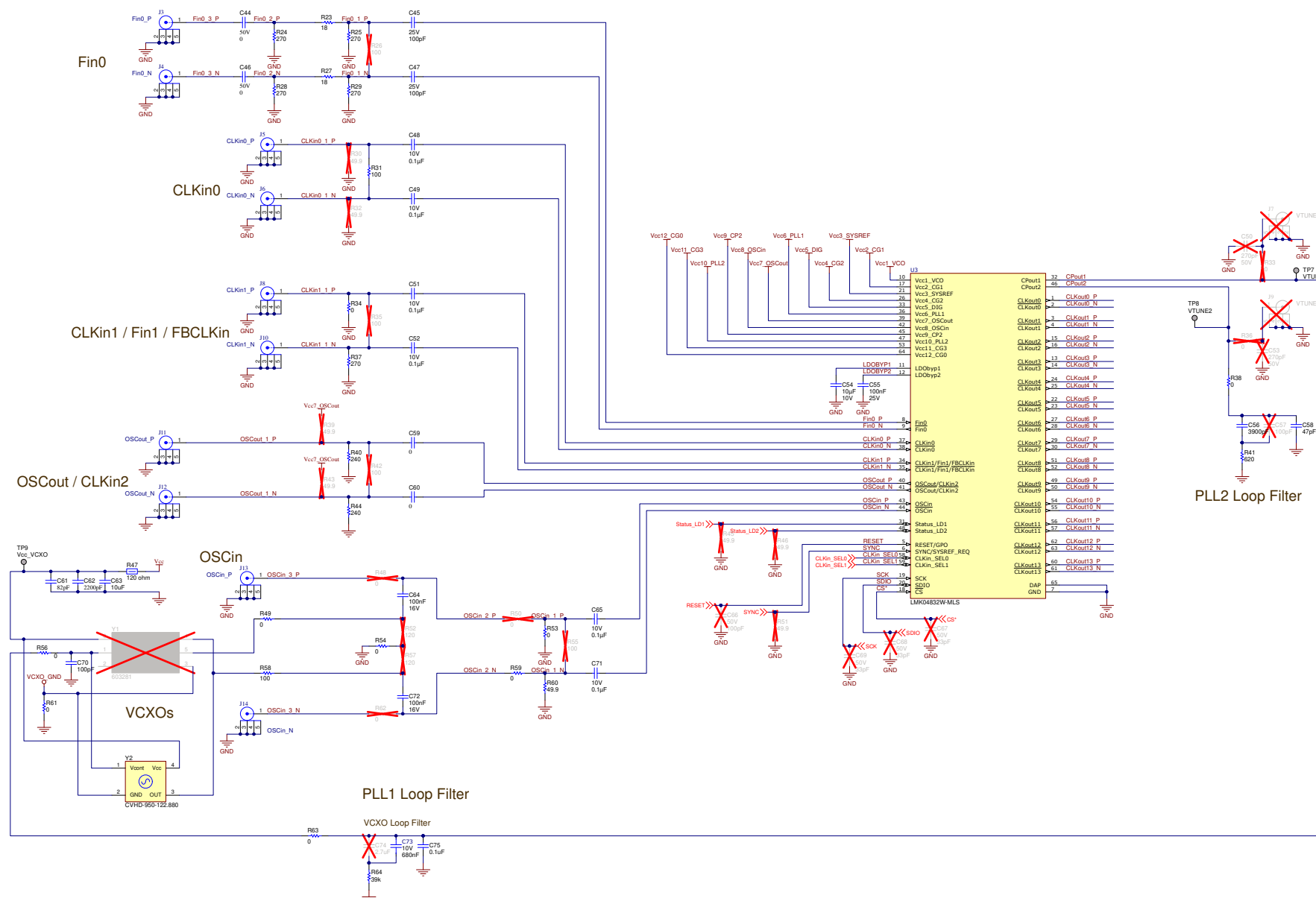
Figure 9. Schematic - LMK04832-SP
