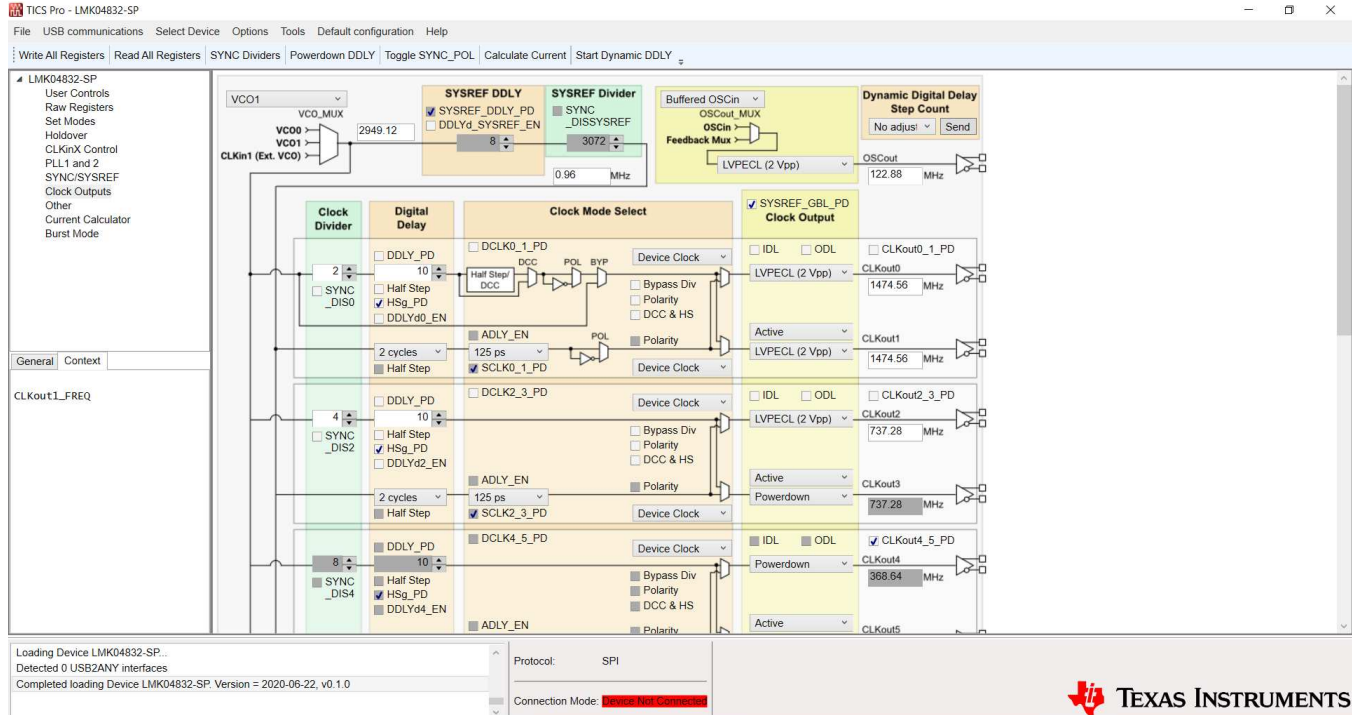
Figure 21. TICS Pro - Clock Outputs Page
