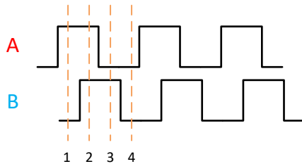
Figure 3. Quadrature Encoding Scheme
