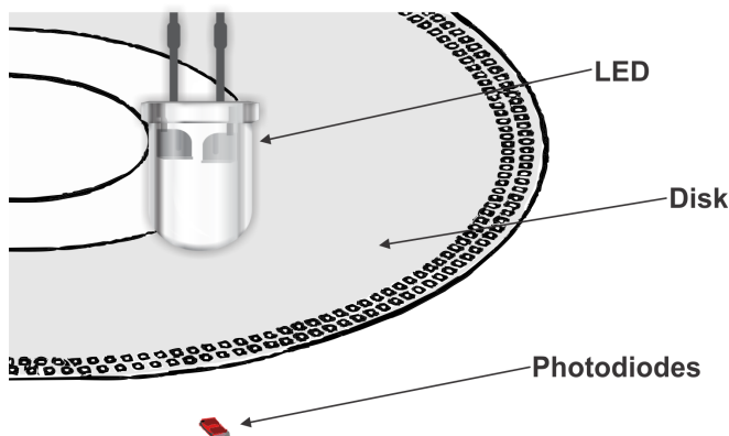
Figure 1. Rotary Motor Shaft Gratings
