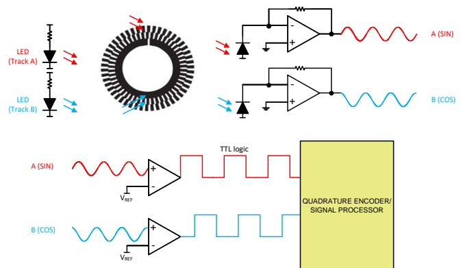
Figure 2. Simplified Incremental Encoder Scheme
