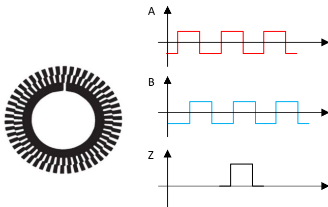
Figure 5. Zero-Reference Signal
