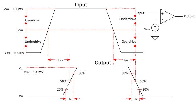
Figure 4. AC Timing Response
