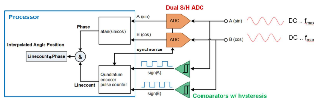
Figure 6. Combined Comparator + ADC Solution
