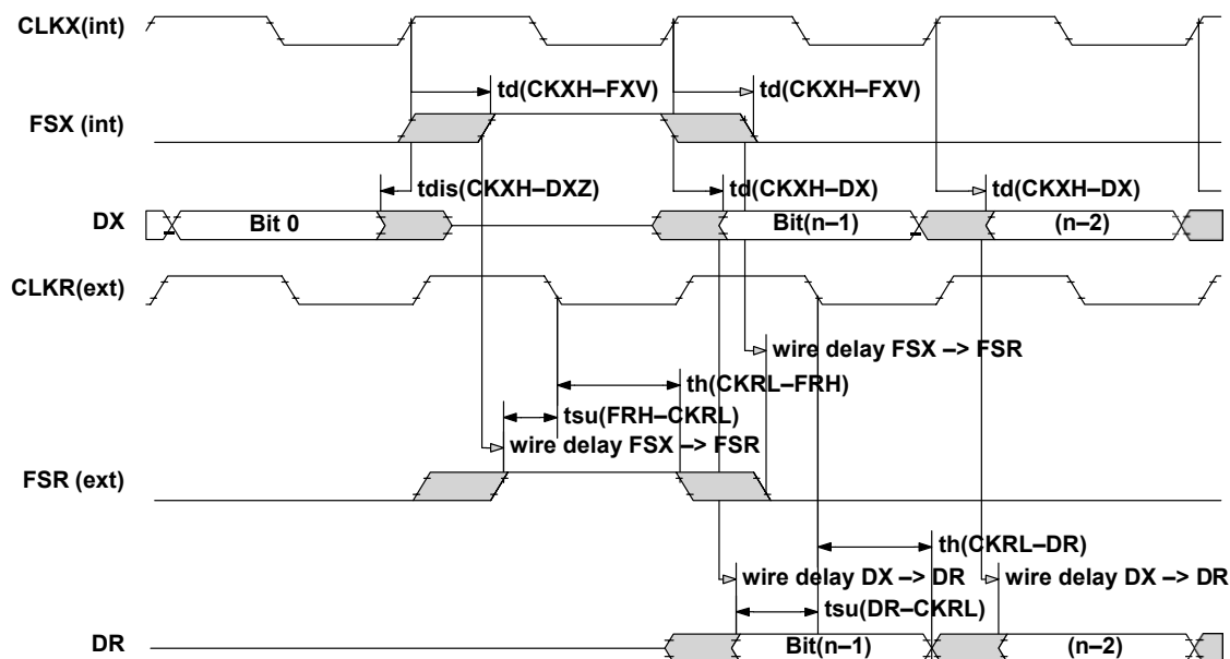
Figure 6. Signal Relationship for C6000 McBSP to McBSP Data Transfer With (R/X)DATDLY=1
