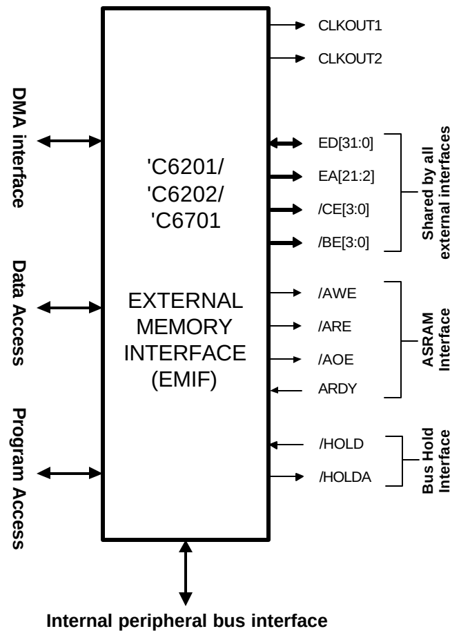
Figure 3. Block Diagram of 'C6201/'C6202/'C6701 EMIF
