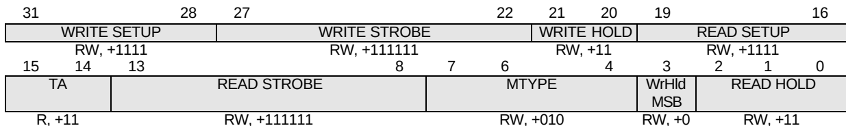
Figure 7. 'C6211'/'C6711 EMIF CE(0/1/2/3) Space Control Register Diagram
