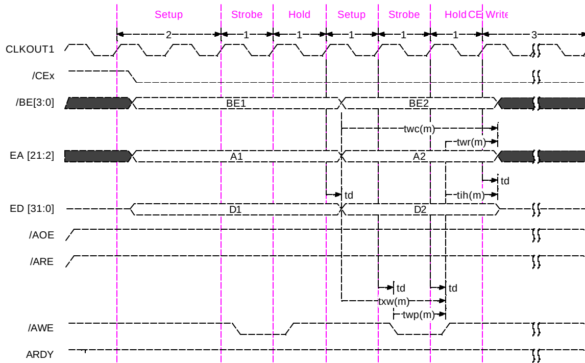
Figure 10. 'C6201/'C6202/'C6701 Asynchronous Write Timing Example (1/1/1)
