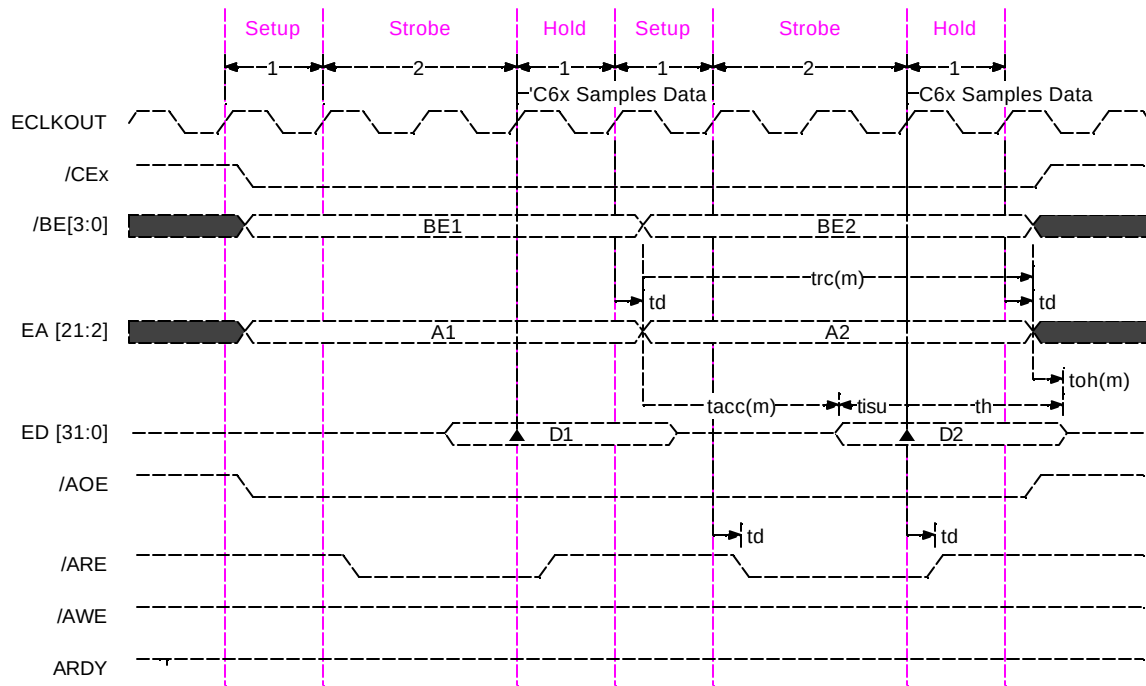
Figure 9. 'C6211/'C6711 Asynchronous Read Timing Example (1/2/1)
