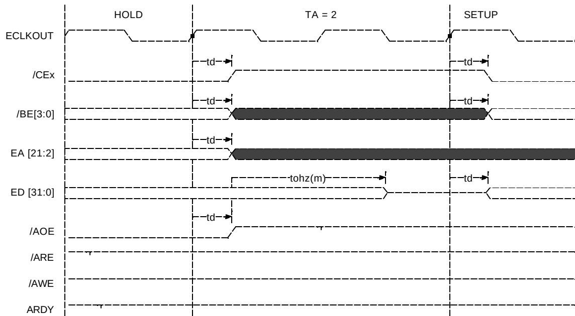
Figure 12. Turnaround Time on 'C6211'/C6711
