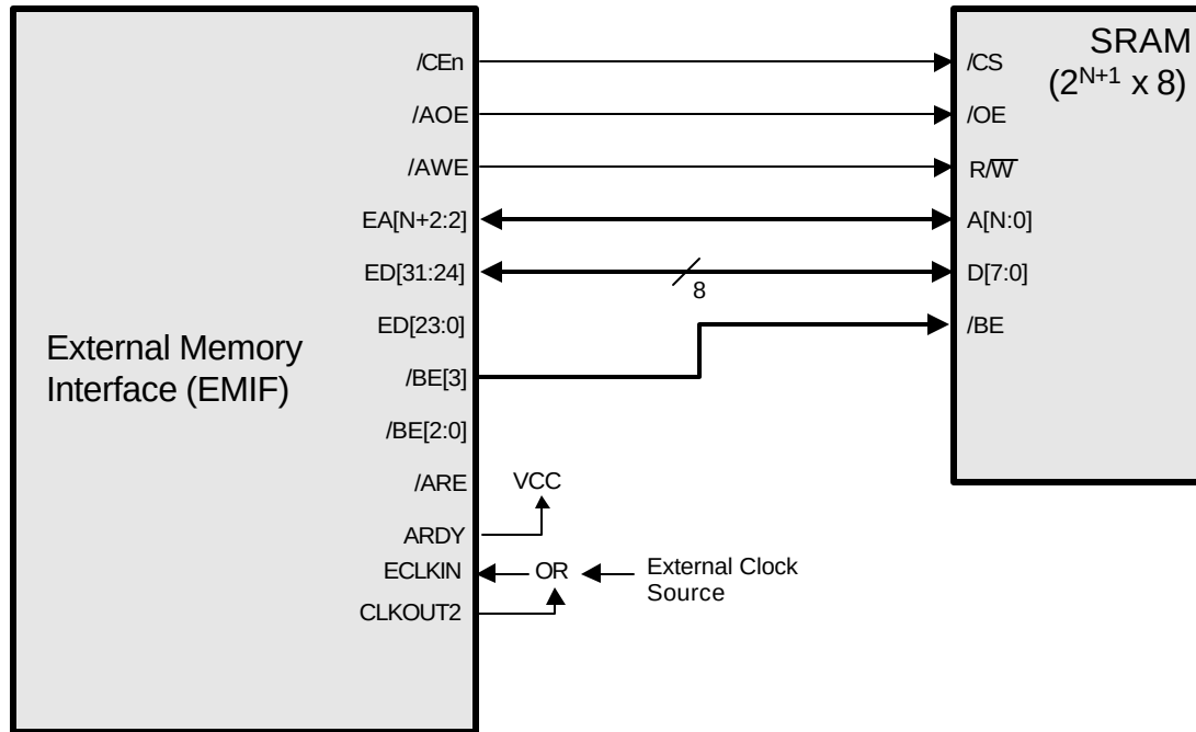
Figure 2. EMIF—Big-Endian x8 ASRAM Interface ('C6211/'C6711 Only)
