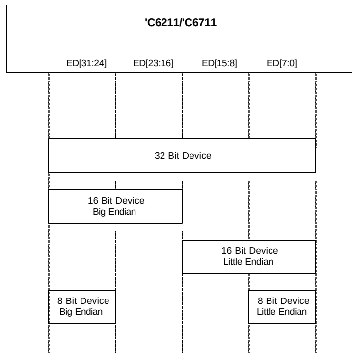
Figure 5. Byte Lane Alignment vs. Endianness on the 'C6211/'C6711
