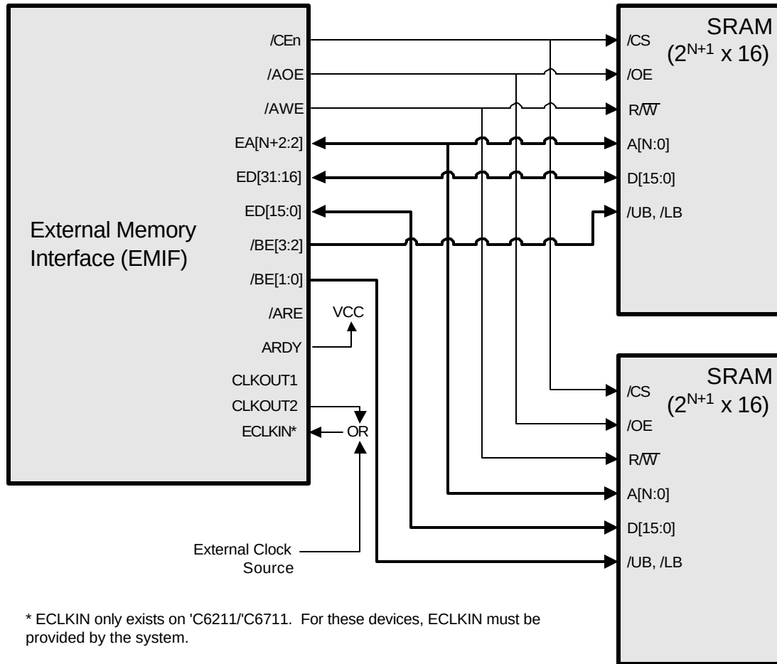
Figure 1. EMIF-SRAM Interface (All C6000 Devices)
