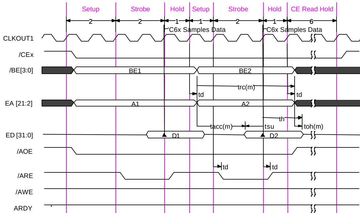
Figure 8. 'C6201/'C6202/'C6701 Asynchronous Read Timing Example (1/2/1)
