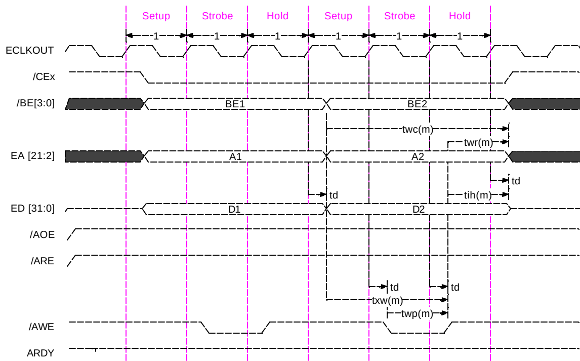
Figure 11. 'C6211/'C6711 Asynchronous Write Timing Example (1/1/1)
