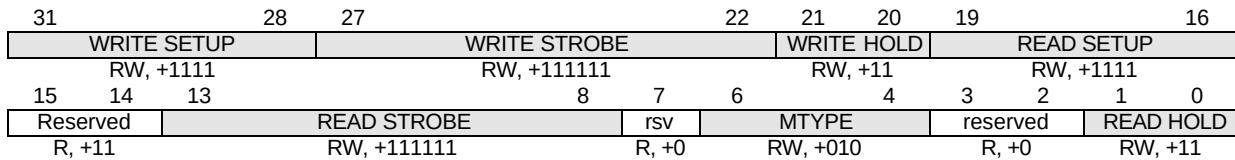
Figure 7. 'C6211'/'C6711 EMIF CE(0/1/2/3) Space Control Register Diagram
