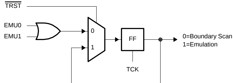
Figure 1. Internal Circuitry for JTAG Operation Mode Select
