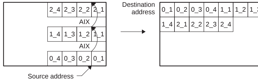
Figure A–76. Array Synchronized 2D-to-1D Transfer (SUM = 10, DUM = 01)
