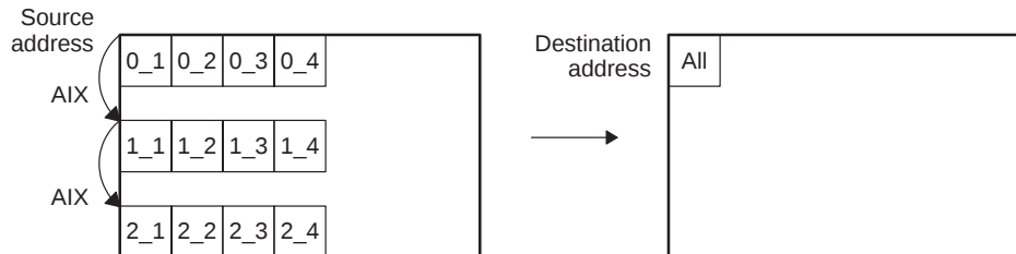
Figure A–72. Array Synchronized 2D-to-1D Transfer ( SUM = 01 , DUM = 00 )
