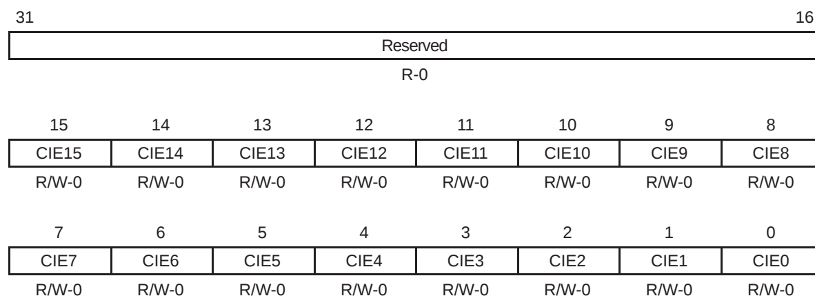
Figure 3–7. EDMA Channel Interrupt Enable Register (CIER)
