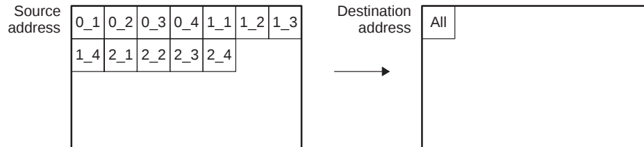
Figure A–63. Block Synchronized 1D-to-2D Transfer ( SUM = 01, DUM = 00)
