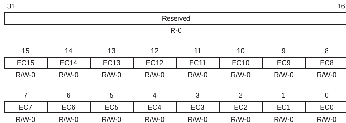
Figure 3–11. EDMA Event Clear Register (ECR)
