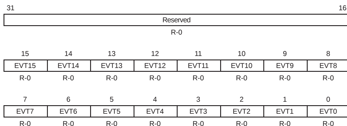
Figure 3–9. EDMA Event Register (ER)
