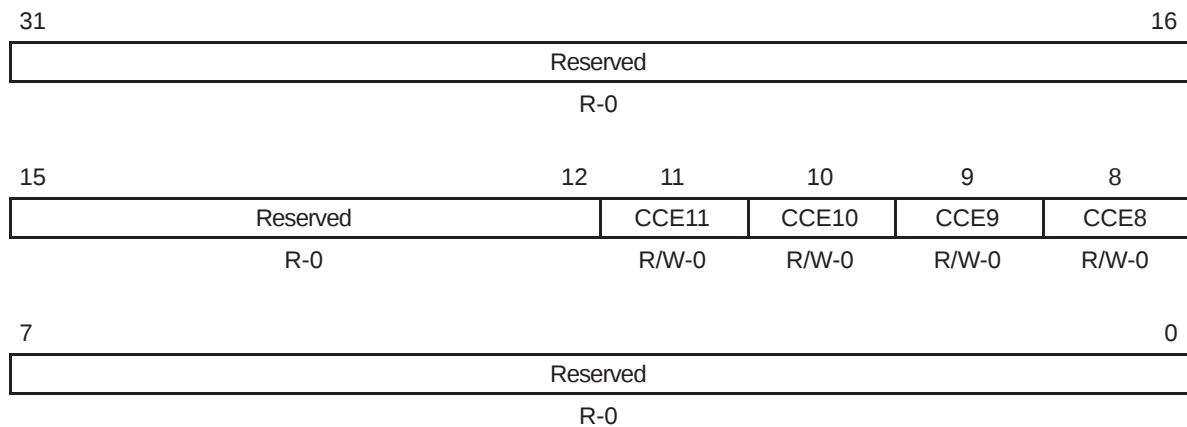
Figure 3–8. EDMA Channel Chain Enable Register (CCER)
