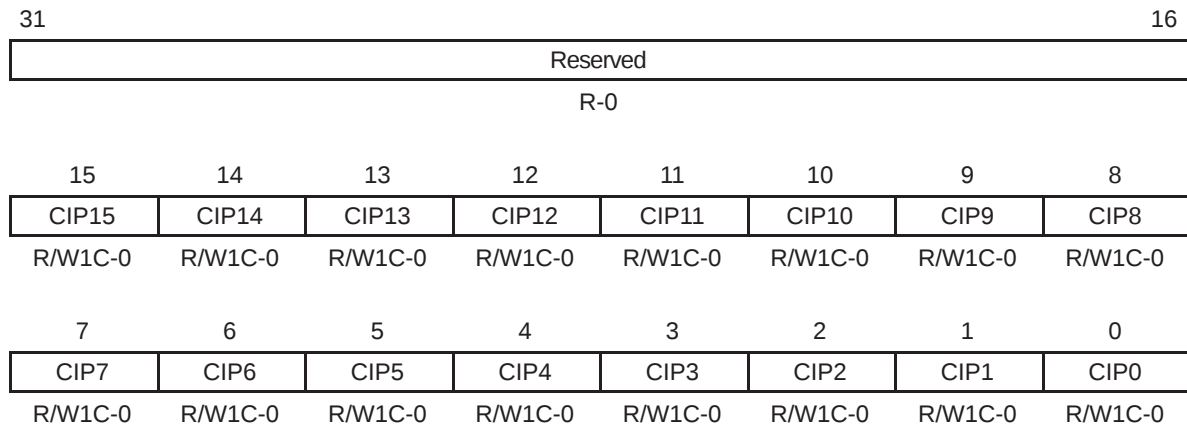
Figure 3–6. EDMA Channel Interrupt Pending Register (CIPR)
