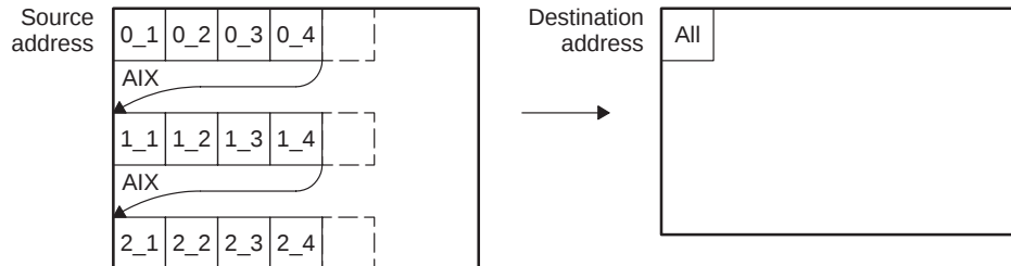
Figure A–81. Block Synchronized 2D-to-1D Transfer ( SUM = 01, DUM = 00)
