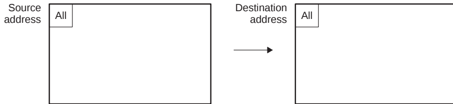
Figure A-51. Array Synchronized 1D-to-2D Transfer (SUM = 00, DUM = 00)
