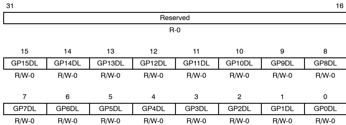
Figure 15. GPIO Delta Low Register (GPD_L)
