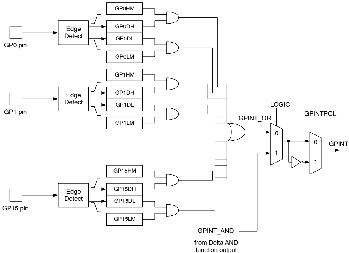
Figure 7. GPINT Generation in Delta OR Mode
