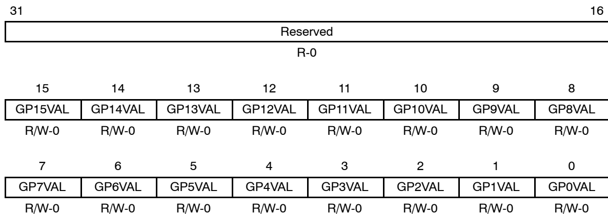
Figure 13. GPIO Value Register (GPVAL)
