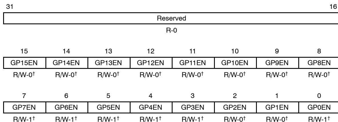
Figure 11. GPIO Enable Register (GPEN)
