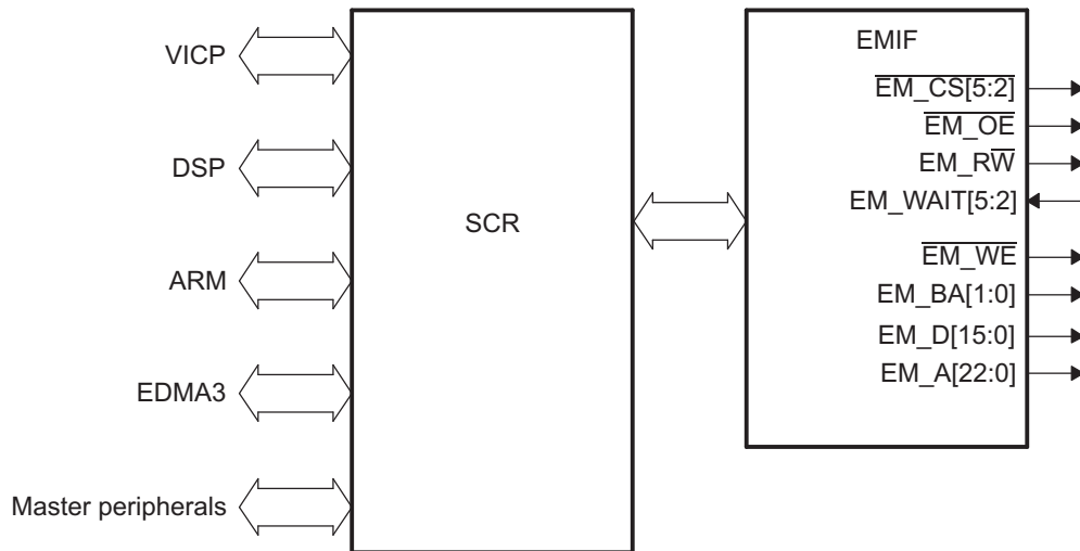
Figure 1. EMIF Functional Block Diagram
