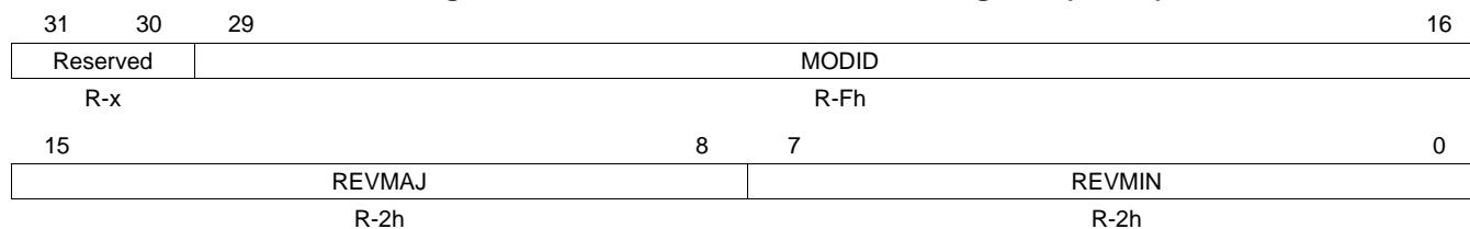
Figure 20. Revision Code and Status Register (RCSR)
