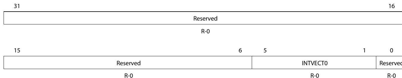
Figure 3-16 SPI Interrupt Vector Register 0 (INTVECO)
