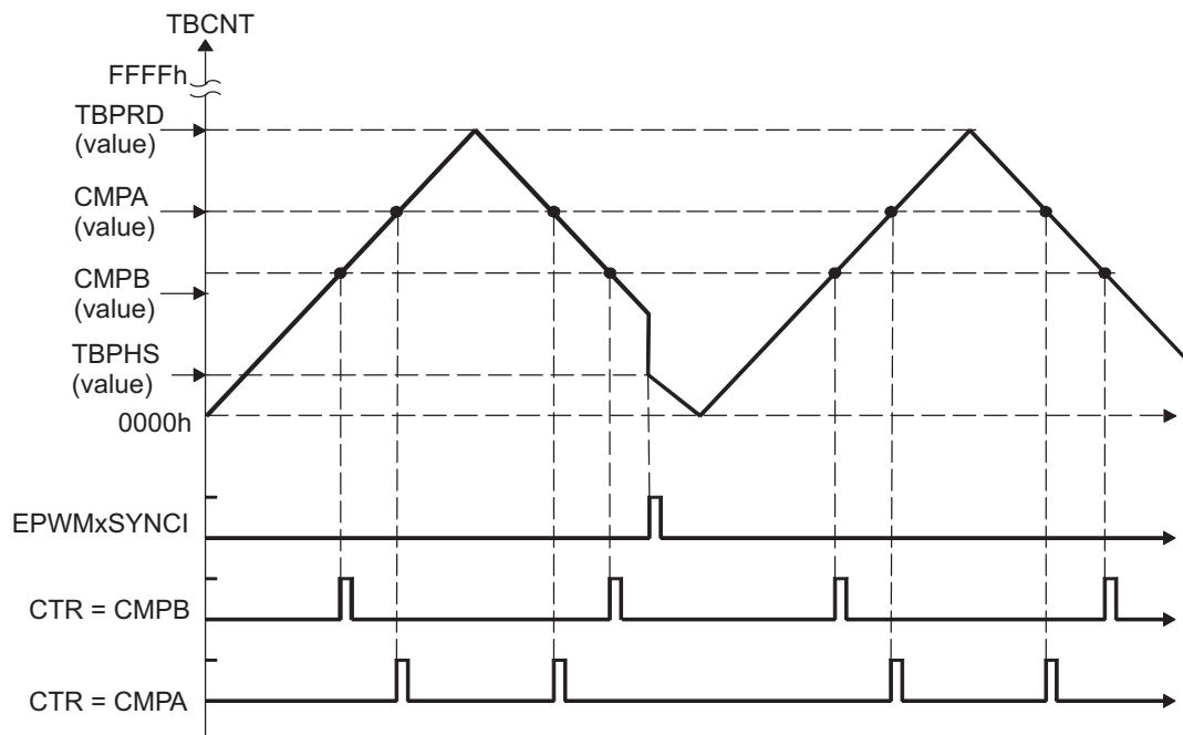
Figure 15-16. Counter-Compare Events in Up-Down-Count Mode, TBCTL[PHSDIR = 0] Count Down on Synchronization Event
