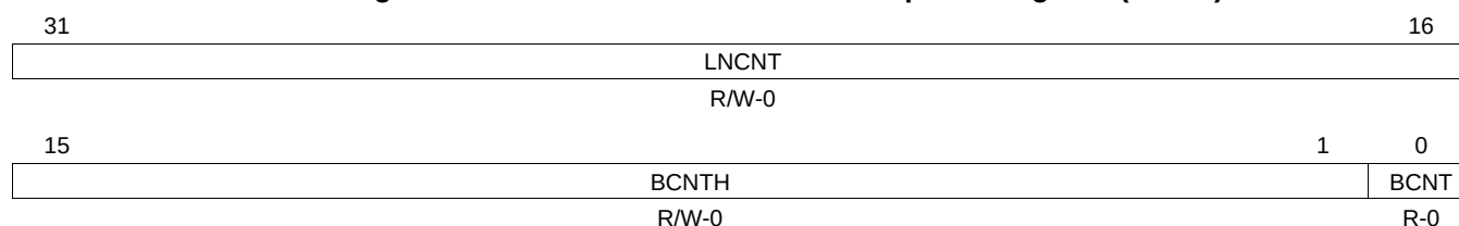
Figure 31-29. uPP DMA Channel I Descriptor 1 Register (UPID1)
