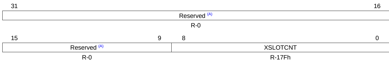
Figure 23-67. Current Transmit TDM Time Slot Register (XSLOT)
