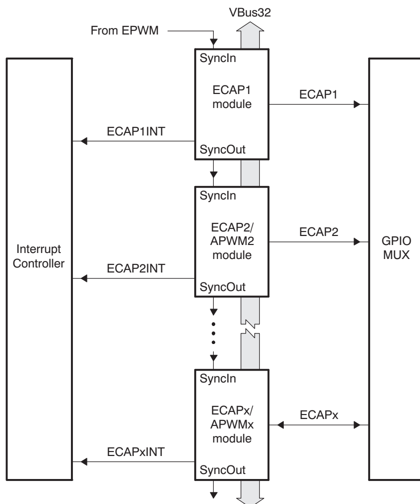
Figure 14-1. Multiple eCAP Modules
