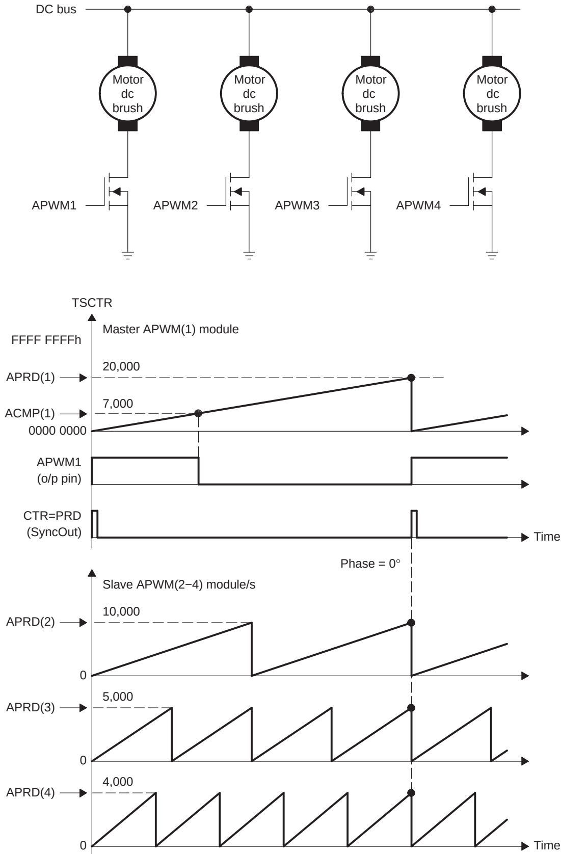
Figure 14-15. Multichannel PWM Example Using 4 eCAP Modules
