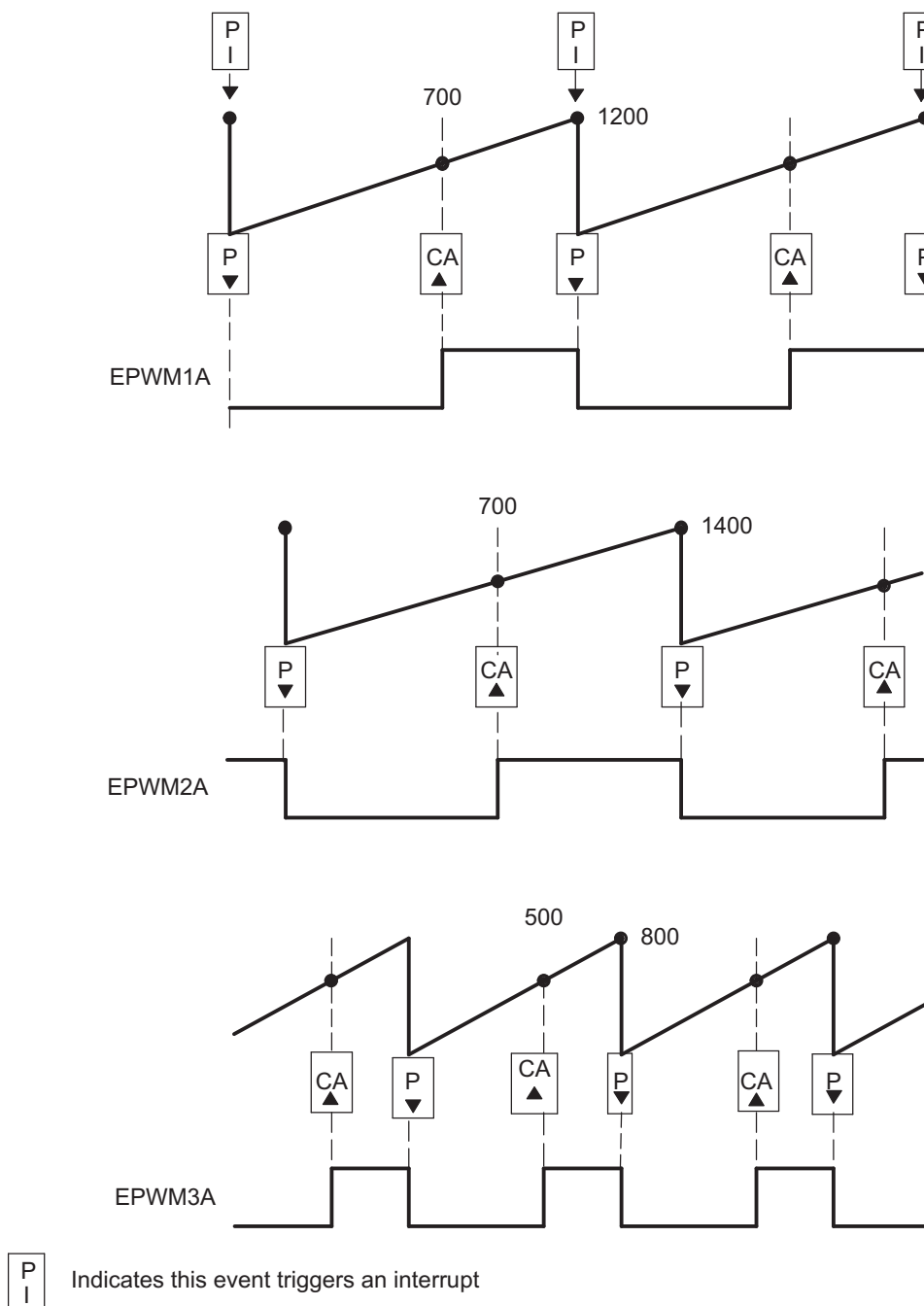
Figure 15-52. Buck Waveforms for Figure 15-51 (Note: Only three bucks shown here)
