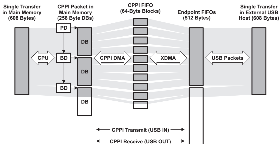
Figure 33-20. High-Level Transmit and Receive Data Transfer Example
