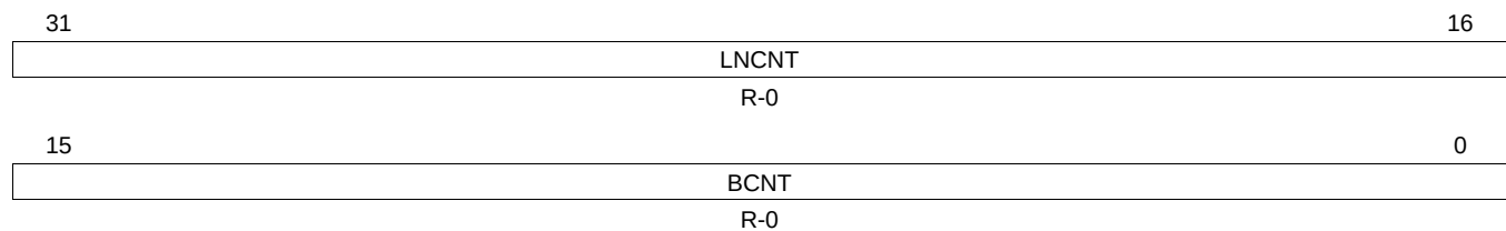
Figure 31-38. uPP DMA Channel Q Status 1 Register (UPQS1)
