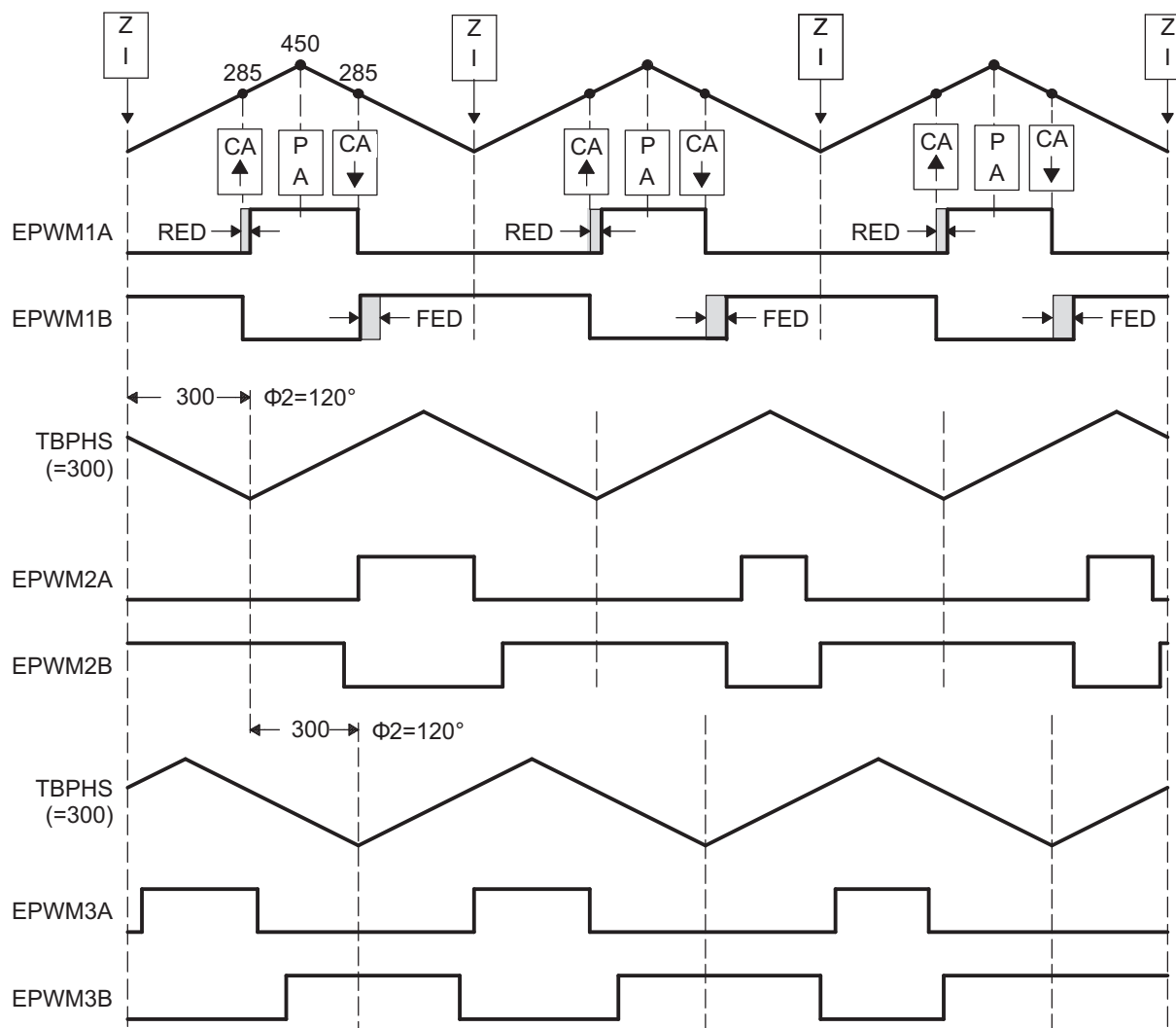
Figure 15-62. 3-Phase Interleaved DC/DC Converter Waveforms for Figure 15-61
