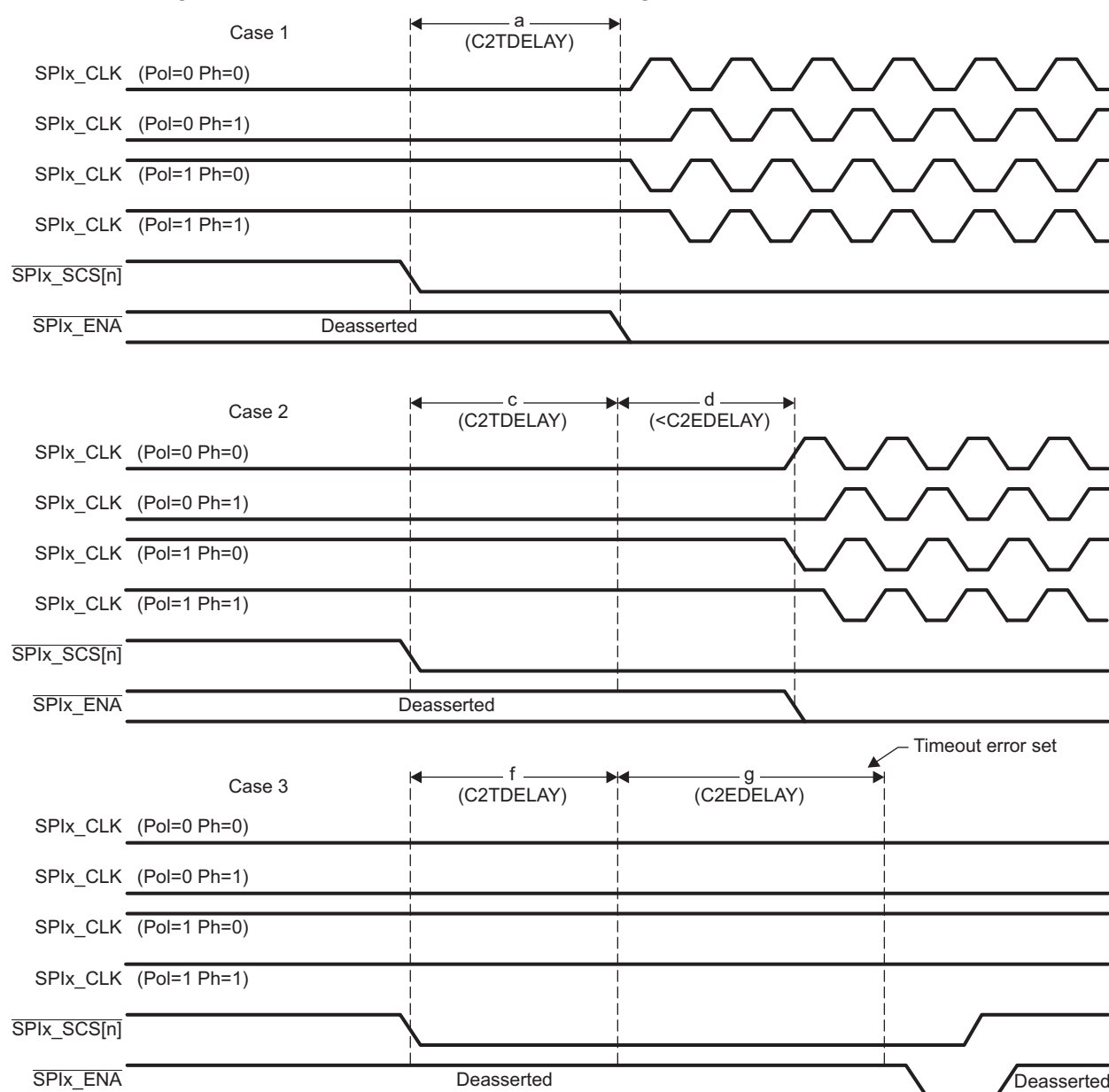
Figure 28-17. SPI 5-Pin Mode Demonstrating C2TDELAY and C2EDELAY
