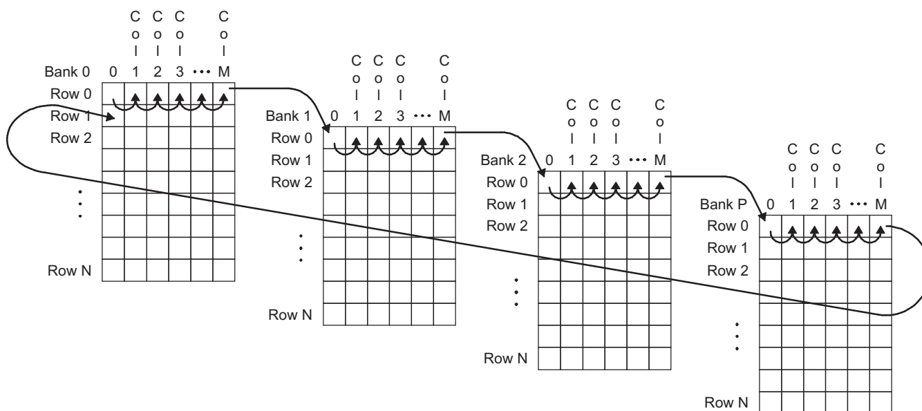
Figure 13-12. DDR2/mDDR SDRAM Column, Row, and Bank Access
