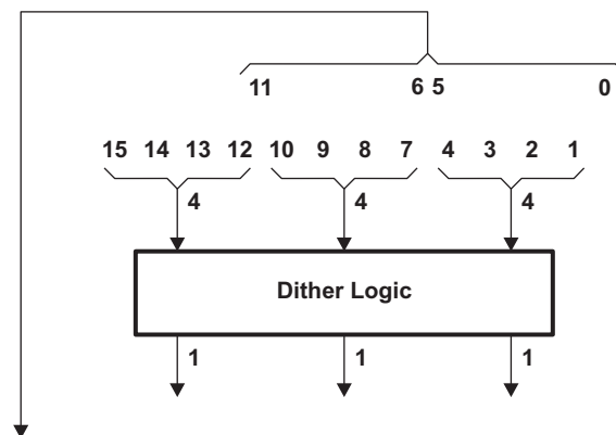
Figure 22-29. 16-BPP STN Mode
