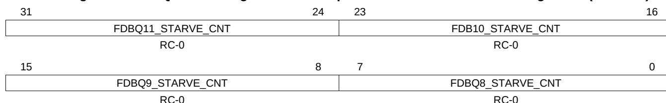
Figure 33-105. Queue Manager Free Descriptor/Buffer Starvation Count Register 2 (FDBSC2)
