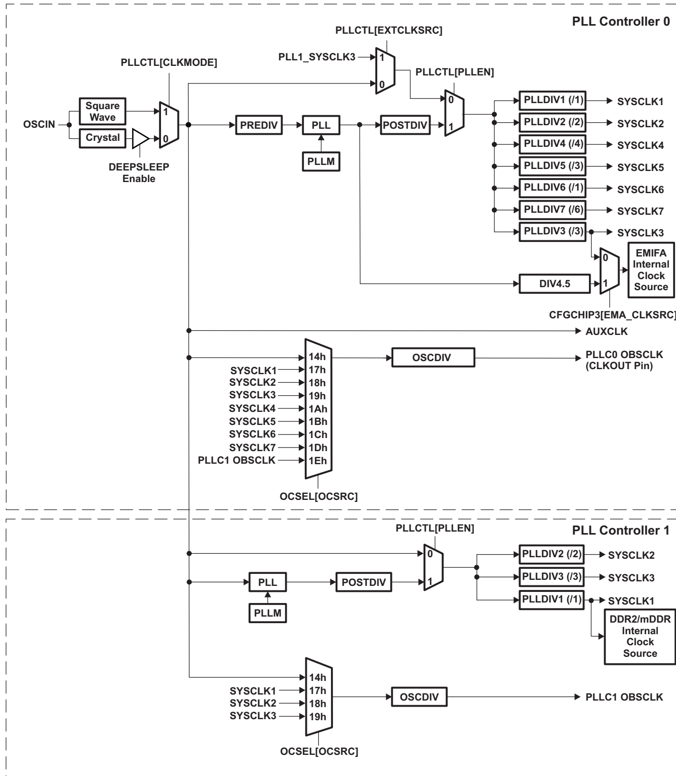
Figure 7-1. PLLC Structure
