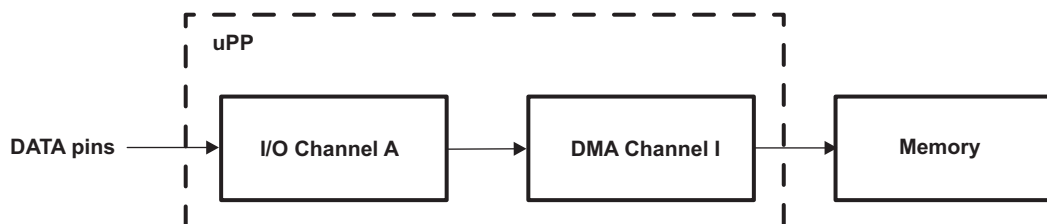
Figure 31-2. Data Flow for Single-Channel Receive Mode
