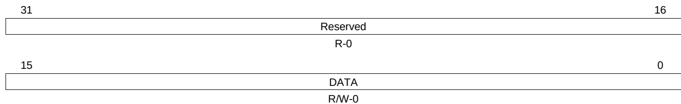
Figure 22-21. LCD LIDD CS n Data Read/Write Register (LIDD_CS n _DATA)
