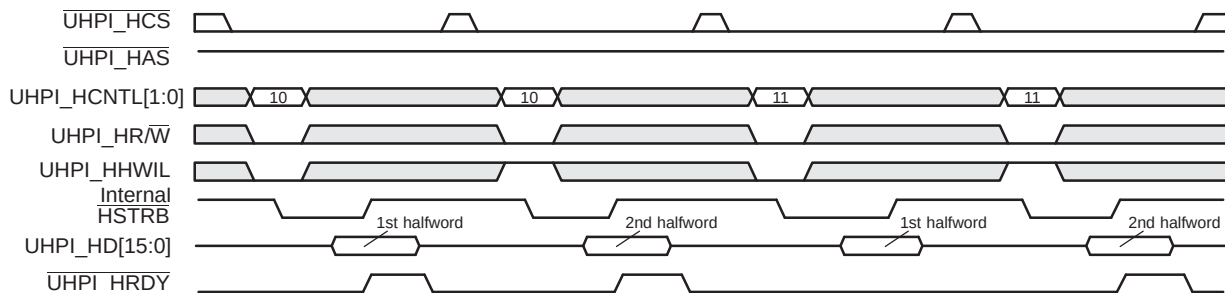
Figure 20-11. \overline{\text{UHPI\_HRDY}} Behavior During a Data Write Operation in the Multiplexed Mode (Case 1: No Autoincrementing)
