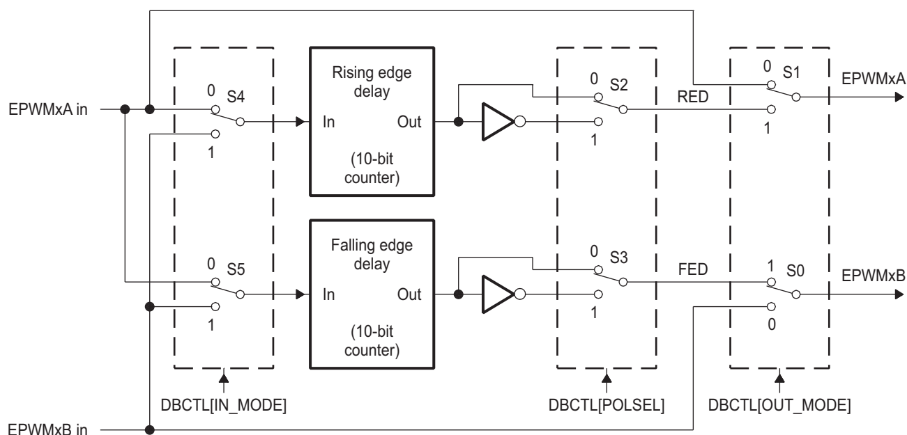
Figure 15-29. Configuration Options for the Dead-Band Generator Submodule
