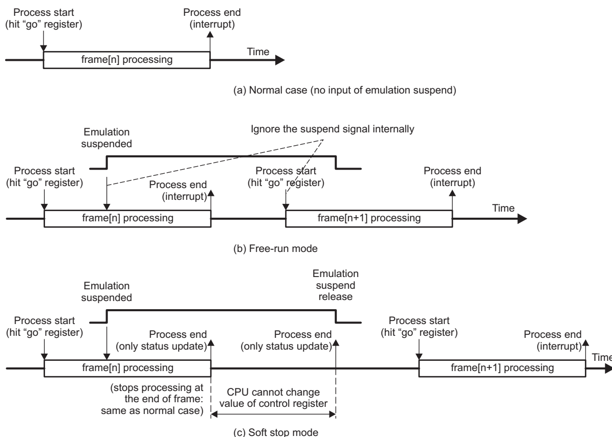
Figure 34-12. Module Performance with Emulation Suspend Signal
