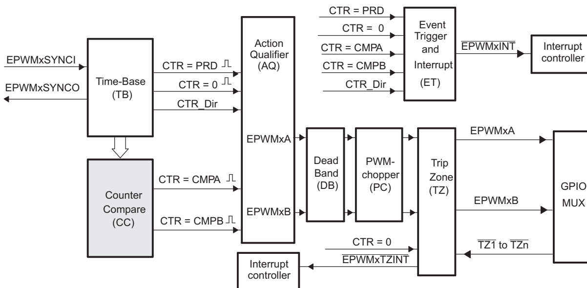
Figure 15-12. Counter-Compare Submodule
