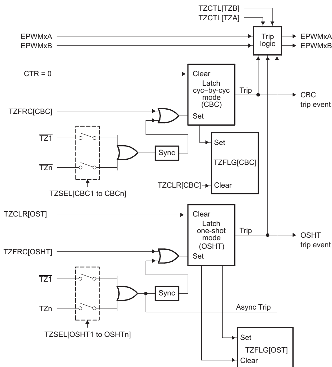
Figure 15-37. Trip-Zone Submodule Mode Control Logic
