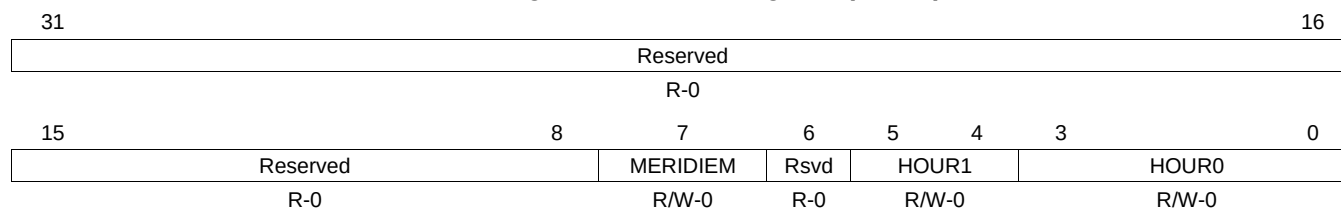
Figure 26-6. Hour Register (HOUR)
