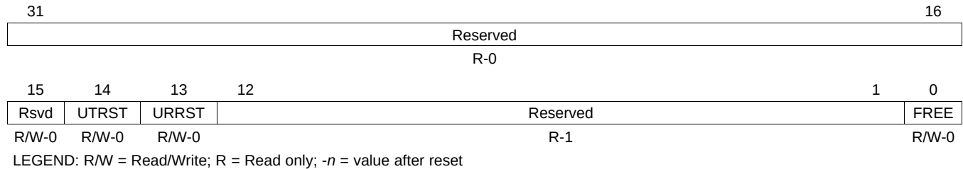
Figure 30-23. Power and Emulation Management Register (PWREMU_MGMT)
