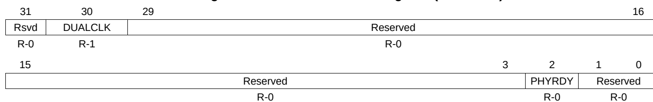
Figure 13-20. SDRAM Status Register (SDRSTAT)
