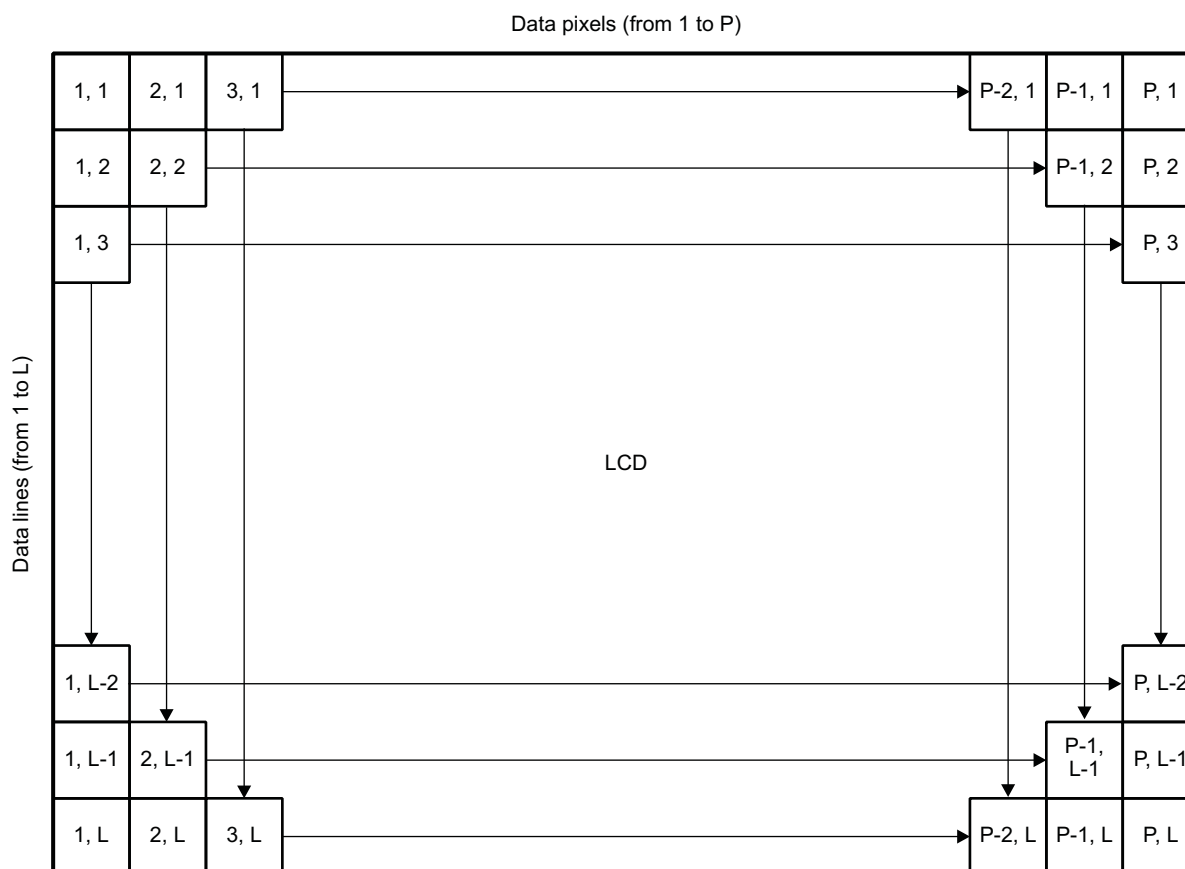
Figure 22-14. Raster Mode Display Format
