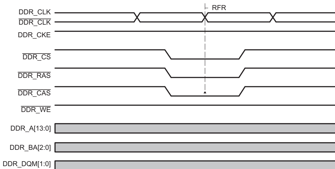
Figure 13-4. Refresh Command
