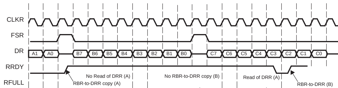
Figure 24-24. Serial Port Receive Overrun Avoided
