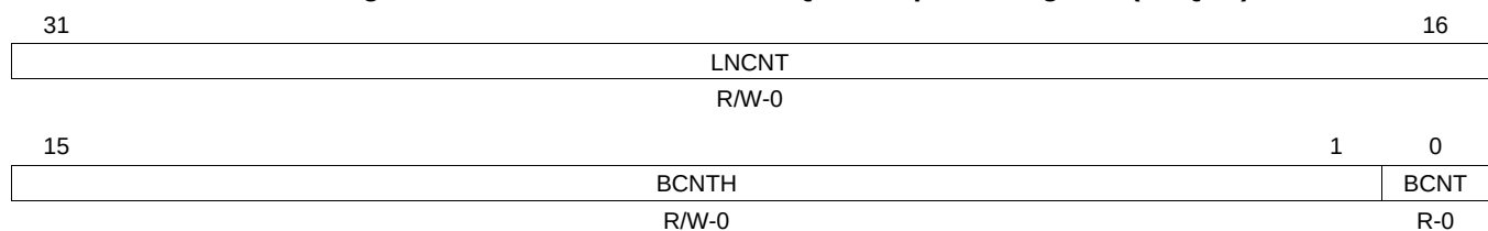
Figure 31-35. uPP DMA Channel Q Descriptor 1 Register (UPQD1)
