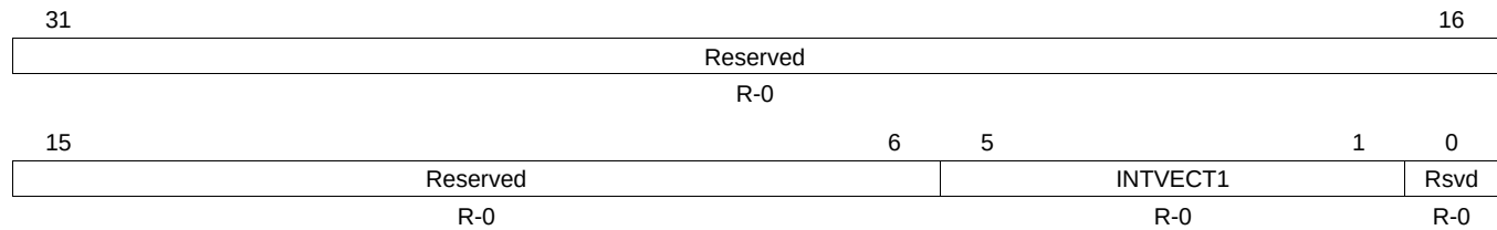
Figure 28-40. SPI Interrupt Vector Register 1 (INTVEC1)
