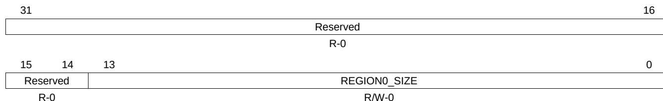
Figure 33-108. Queue Manager Linking RAM Region 0 Size Register (LRAM0SIZE)
