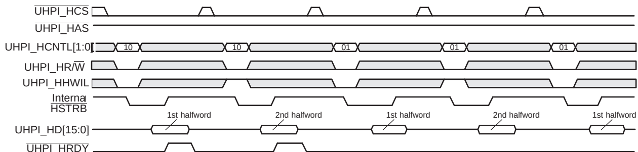
Figure 20-12. \overline{\text{UHPI\_HRDY}} Behavior During a Data Write Operation in the Multiplexed Mode (Case 2: Autoincrementing Selected, FIFO Empty Before Write)
