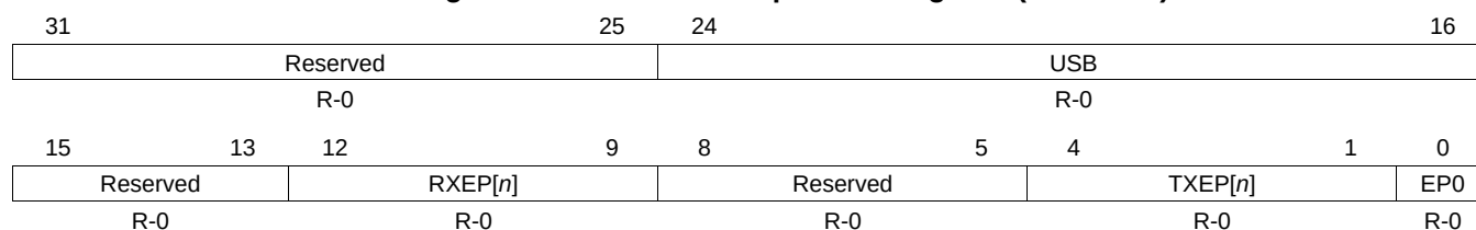
Figure 33-38. USB Interrupt Mask Register (INTMSKR)
