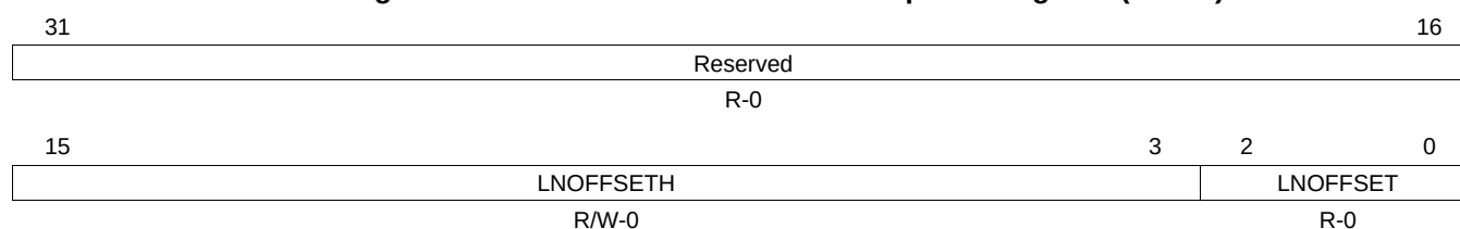
Figure 31-30. uPP DMA Channel I Descriptor 2 Register (UPID2)
