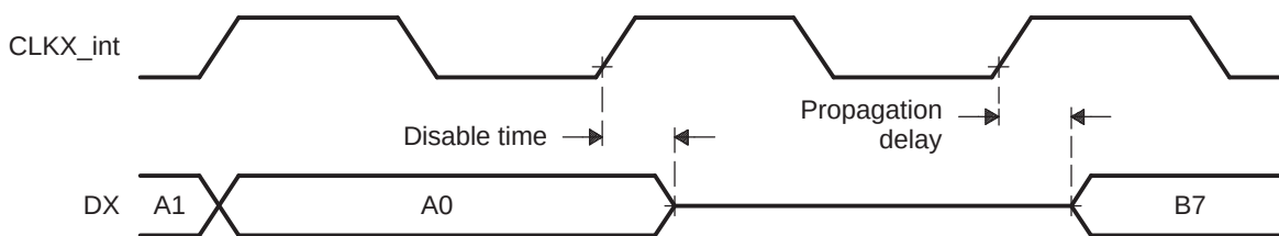
Figure 24-3. Transmit Data Clocking
