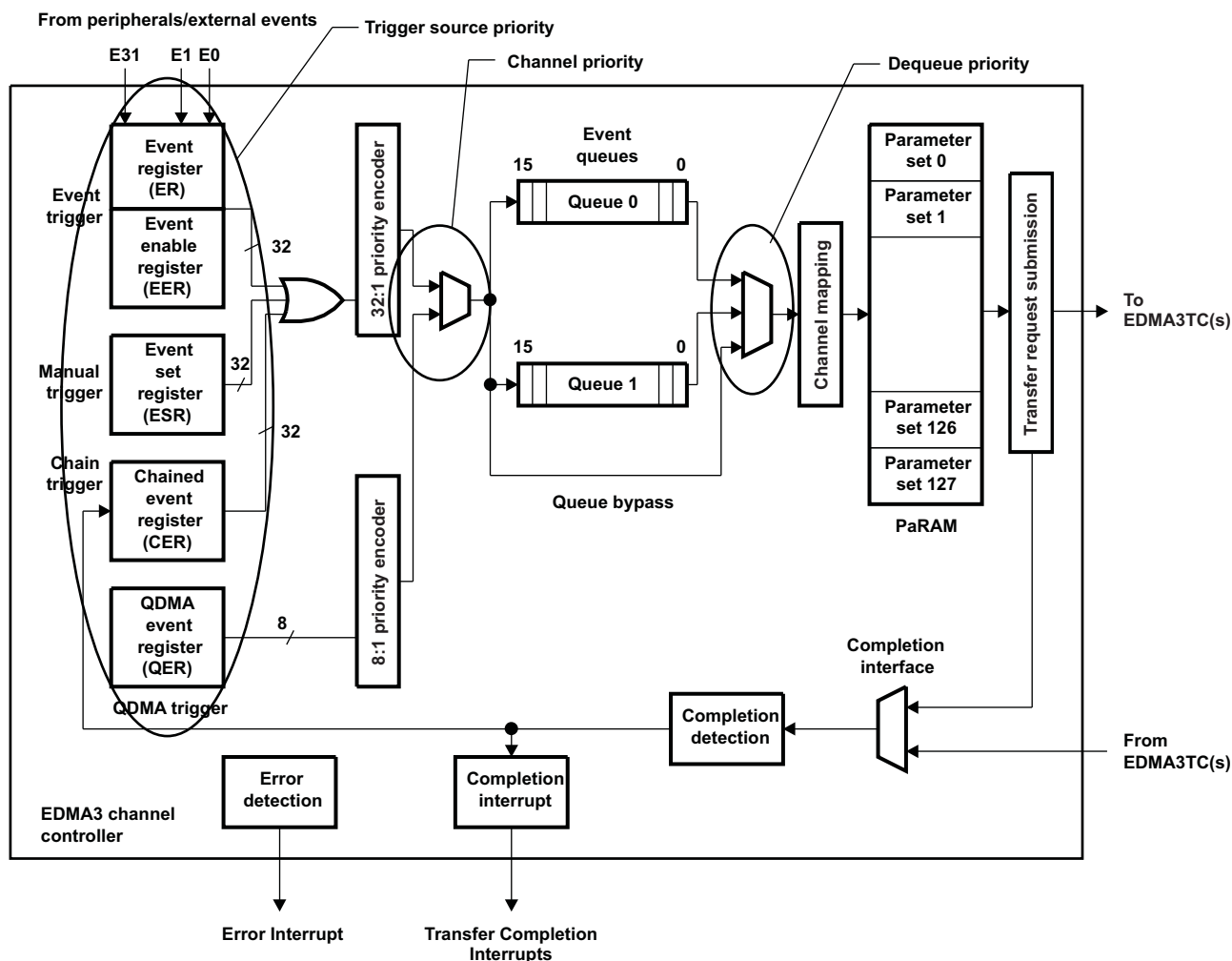
Figure 16-14. EDMA3 Prioritization
