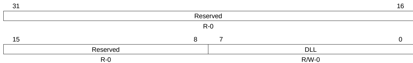
Figure 30-19. Divisor LSB Latch (DLL)
