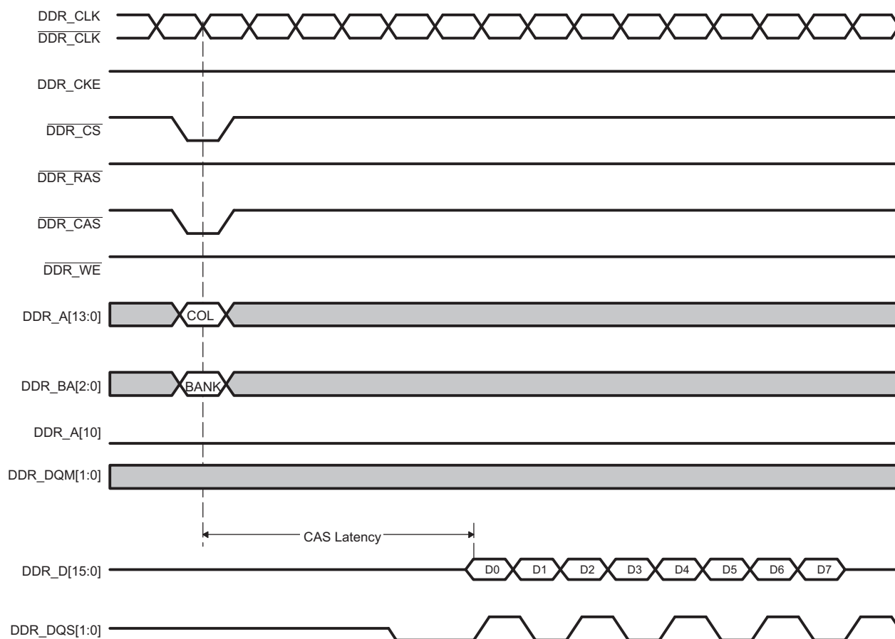
Figure 13-8. DDR2/mDDR READ Command
