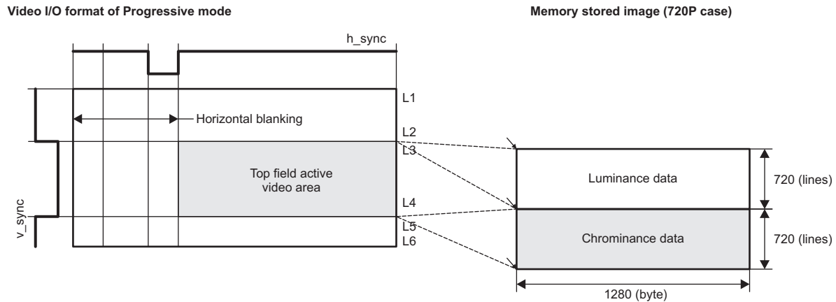
Figure 34-5. Progressive Video
