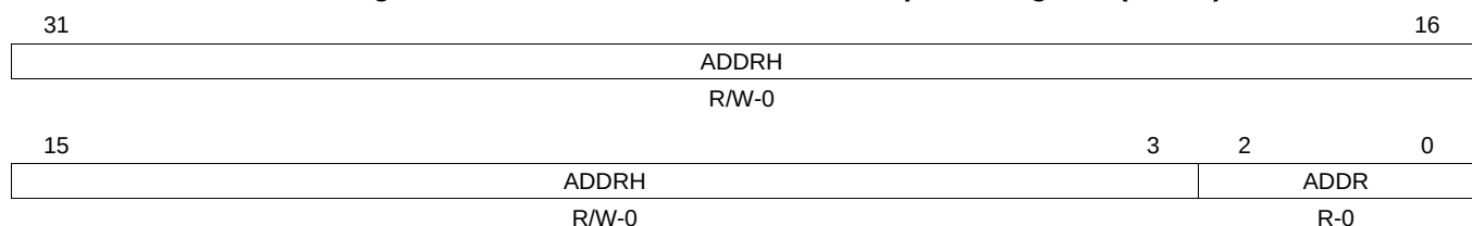
Figure 31-28. uPP DMA Channel I Descriptor 0 Register (UPID0)
