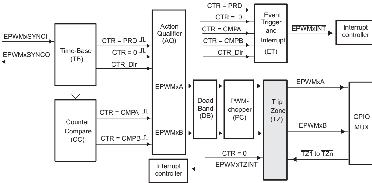
Figure 15-36. Trip-Zone Submodule
