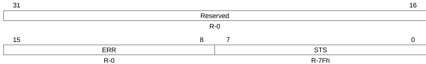
Figure 27-25. Port Task File Data Register (P0TFD)
