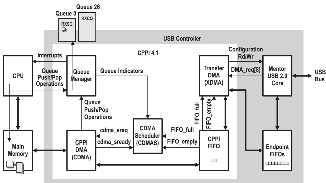
Figure 33-25. Receive USB Data Flow Example (Initialization)
