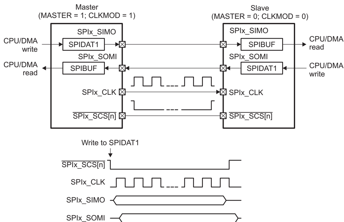
Figure 28-3. SPI 4-Pin Option with \overline{\text{SPIx\_SCS}}[n]
