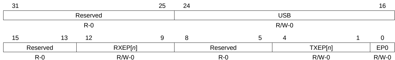
Figure 33-39. USB Interrupt Mask Set Register (INTMSKSETR)
