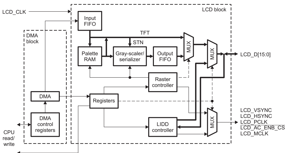
Figure 22-1. LCD Controller
