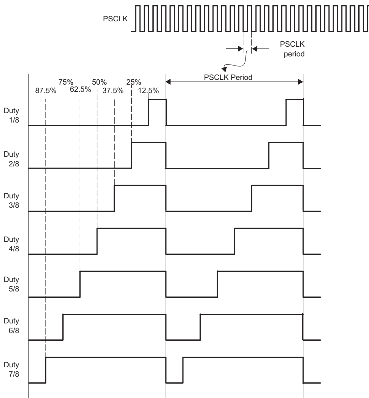
Figure 15-35. PWM-Chopper Submodule Waveforms Showing the Pulse Width (Duty Cycle) Control of Sustaining Pulses
