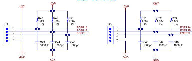
EQEP Connect ors
