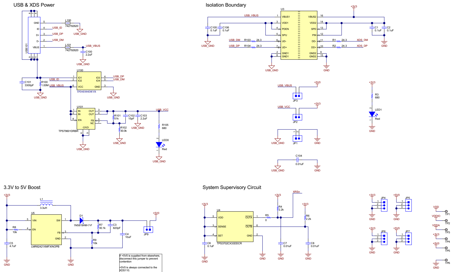
Figure 9. MCU025B_XDS110_USB_Power.SchDoc
