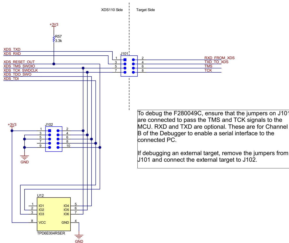
Figure 8. MCU025B_XDS110_Target_Interface.SchDoc
