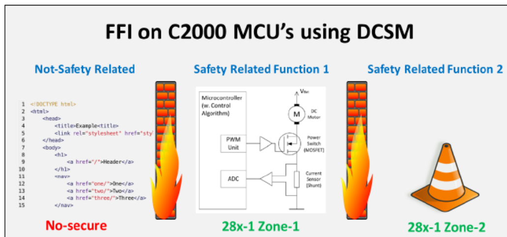
Figure 3. Using DCSM to Prevent Interference
