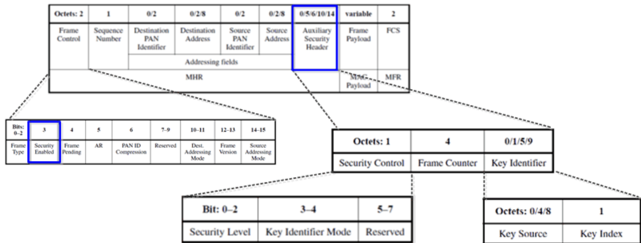
Figure 1. IEEE 802.15.4 Security Header Format
