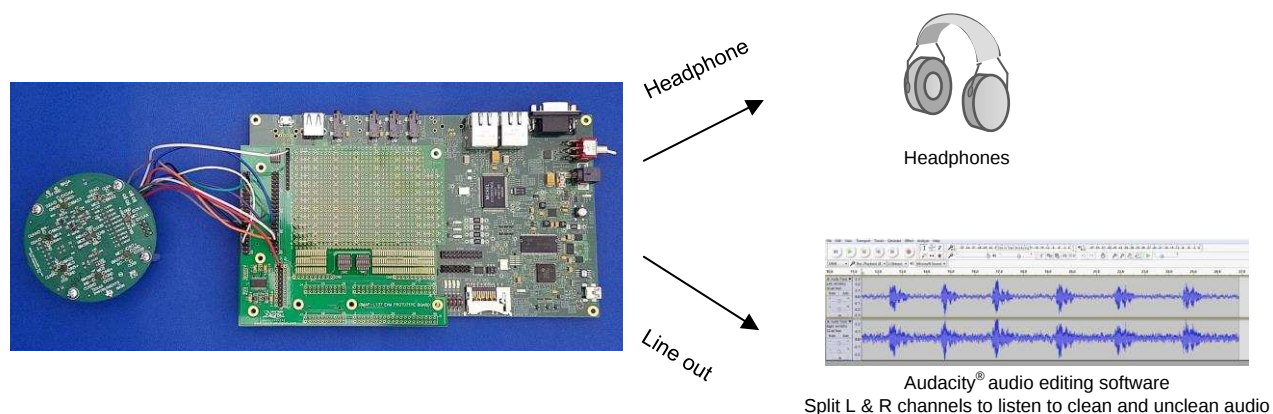
图 12. Overview on Evaluating Audio Output of Voice Pre-processing Demonstration on OMAP-L137/TMS320C6747 Floating Point SK
