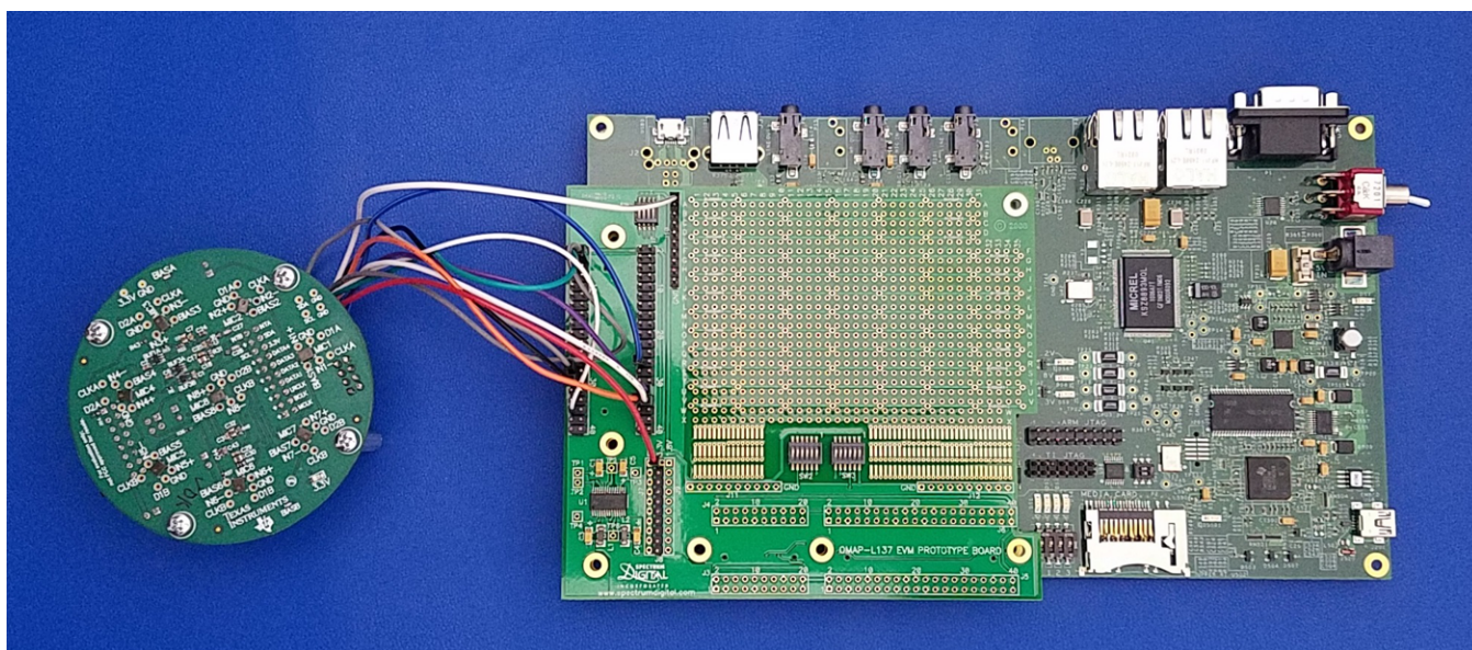
图 10. OMAP-L137/TMS320C6747 Floating Point SK With CMB Connected
