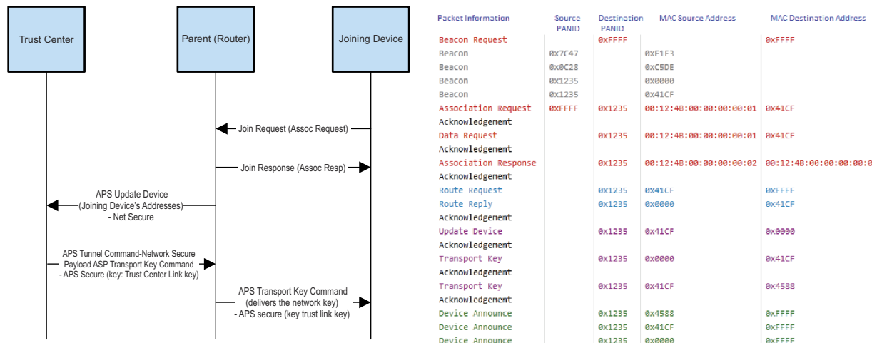
Figure 2-3. (a) Network Join Sequence When the Parent is not the Trust Center (b) Ubiquia Log Snapshot Showing Over the Air Messages During Network Join Procedure
